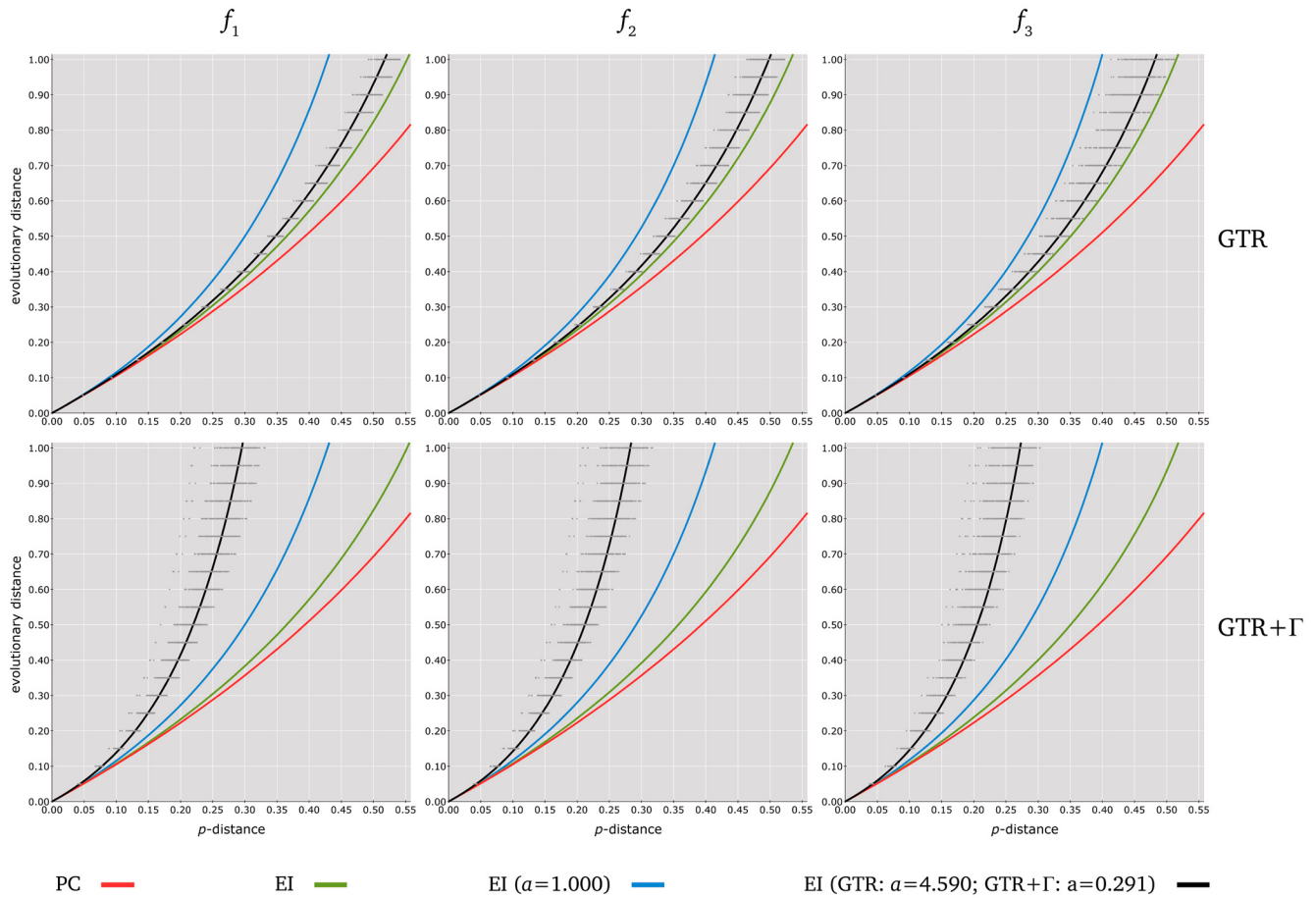
Figure 3. Relationships between p -distances and different evolutionary distance estimates under various models of nucleotide substitution. The six charts represent the evolutionary distance d (y-axis ranging from 0.00 to 1.00) against the p -distance p (x-axis ranging from 0 to 0.55). Gray points ( p, d ) are derived from the simulation of sets of 4,000 sequence pairs, each under six different scenarios of evolution: GTR (top) and GTR+ \Gamma (bottom) with equilibrium frequencies f_1 = (0.25, 0.25, 0.25, 0.25) (left), f_2 = (0.10, 0.30, 0.40, 0.20) (middle) and f_3 = (0.40, 0.10, 0.10, 0.40) (right). PC and EI versions of Equation (2) are represented with red and green curves, respectively. EI version of Equation (3) is represented with blue curves for a = 1 , and with black curves for the values a = 4.590 and a = 0.291 determined by least-square regression from the gray points derived from the models GTR (top) and GTR+ \Gamma (bottom), respectively.
