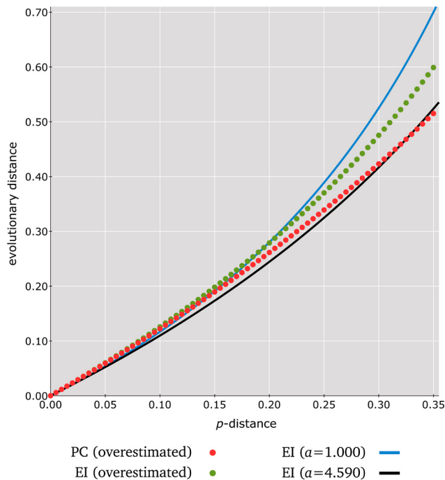
Figure 4. Impact of the MH p -distance upward bias on PC and EI transformations. The relationship between the p -distance p (x-axis ranging from 0.00 to 0.35) and the corresponding evolutionary distance d (y-axis ranging from 0.00 to 0.70) is represented when using PC (red dots) and EI (with equilibrium frequencies f_2 ; green dots) transformations (2) on \hat{p} = \beta p with \beta = 1.15 . For ease of comparison with Figure 3, EI ( f_2 ) transformation (3) on p are represented with a = 1.000 (blue curve) and a = 4.590 (black curve).
