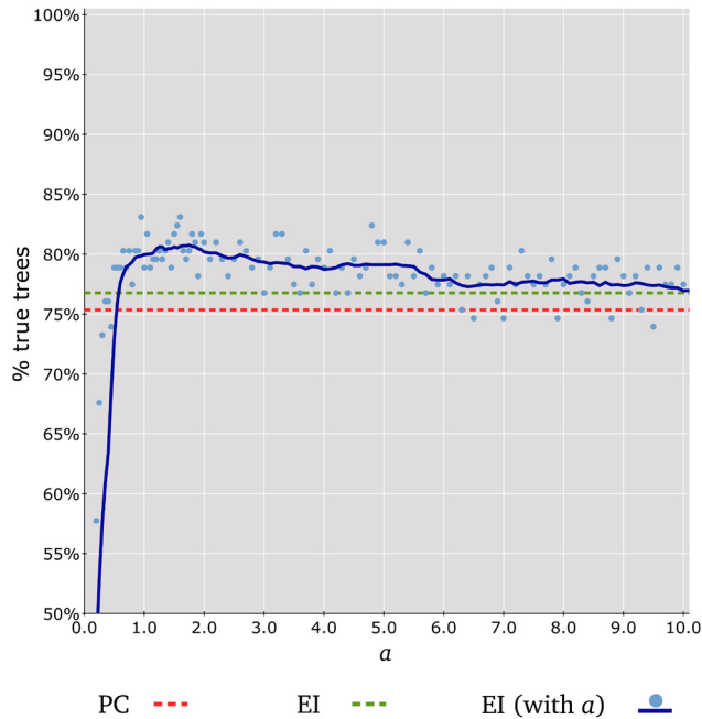
Figure 5. Accuracy of different p -distance transformations for phylogenetic inference. The percentage of recovered reference trees (y-axis ranging from 50% to 100%) is represented (light blue dots) in function of the parameter \alpha (x-axis ranging from 0.0 to 10.0) in EI formula (3). The overall trend of these dots is illustrated using a moving average (dark blue curve). Dashed lines represent the percentages of recovered reference trees obtained with the PC (red) and EI (green) transformations (2).
