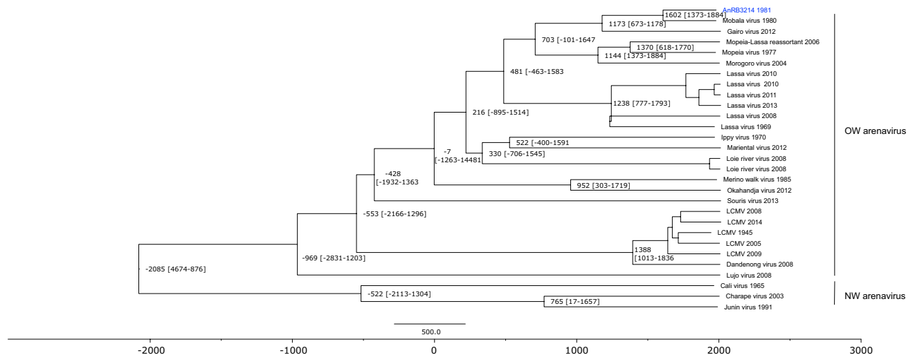
Figure 4. Molecular clock analysis of strain AnRB3214 using BEAST v1.10.4. The clock shows two monophyletic arenavirus groups which seems to have diverged some 5000 years ago. AnRB3214 strain (in blue) diverged from an ancestor in common with Mobala virus around year 1602 [year 1373– year 1884]. BEAST v1.10.4 ( https://www.beast2.org/ ) was used for the Bayesian Monte Carlo Markov chain (MCMC) inference and the chronogram was generated with TreeAnnotator v1.10.4 ( https://beast.community/treeannotator ).
