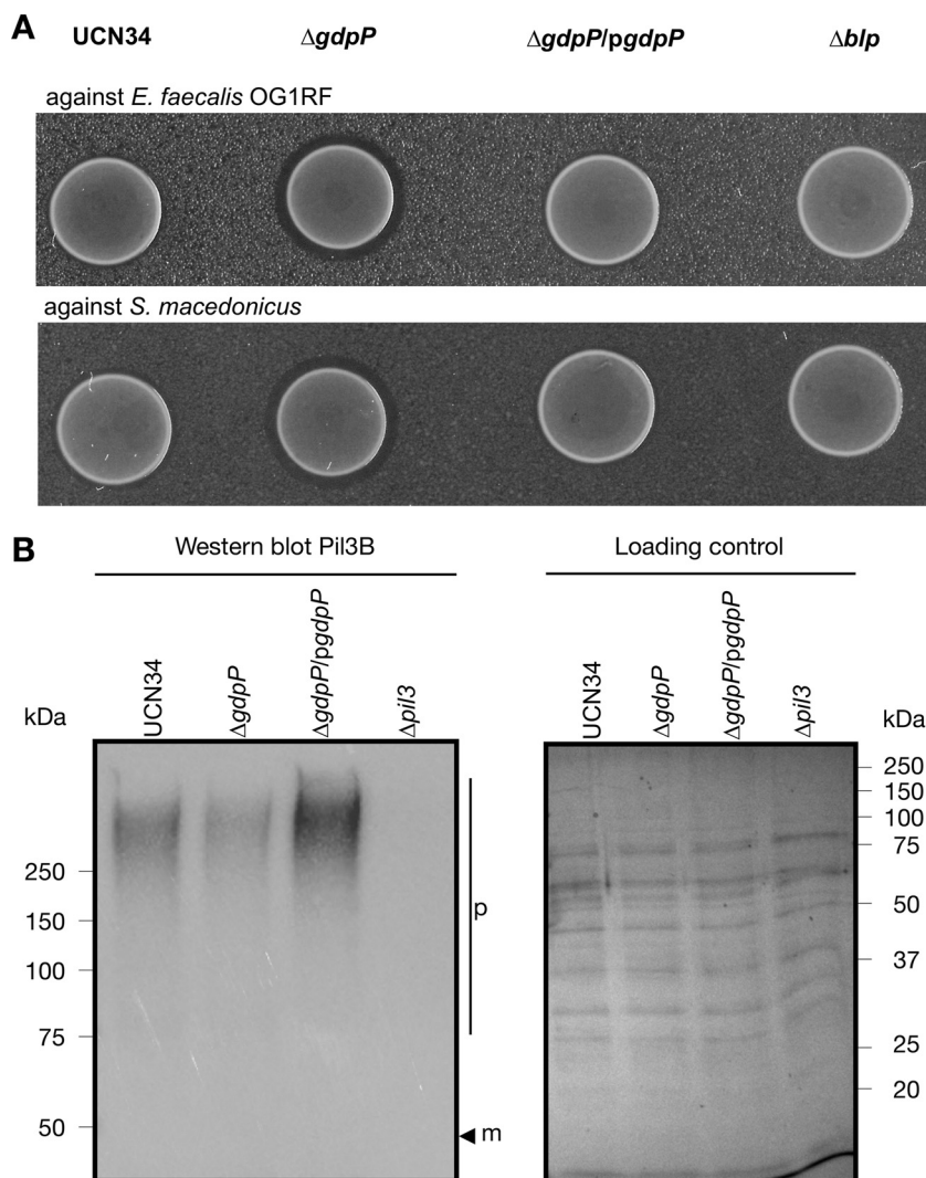
FIG 5 c-di-AMP regulates the gallocin production and Pil3 biosynthesis in S. gallolyticus subsp. gallolyticus . (A) Gallocin production by S. gallolyticus subsp. gallolyticus UCN34, the \Delta gdpP mutant, and the \Delta gdpP/pgdpP complemented strain under anaerobic conditions. Five microliters of S. gallolyticus subsp. gallolyticus UCN34, the \Delta gdpP mutant, and the \Delta gdpP/pgdpP complemented strain log-phase culture adjusted to approximately 3 \times 10^7 CFU/ml was spotted onto BHI agar flooded with Enterococcus faecalis OG1RF or S. gallolyticus subsp. macedonicus . Zone of clearance reflects the growth inhibition of E. faecalis or S. gallolyticus subsp. macedonicus . The strain deficient in producing the gallocin \Delta blp mutant was used as the negative control. (B) Western blot analysis of the cell wall proteins from S. gallolyticus subsp. gallolyticus UCN34, the \Delta gdpP mutant, and the \Delta gdpP/pgdpP complemented strain. Equal amounts of the cell wall proteins were loaded (right) and probed with specific polyclonal antibodies against Pil3B (left). Cell wall proteins of the S. gallolyticus subsp. gallolyticus UCN34 \Delta pil3 mutant was used as a negative control. Theoretical positions of Pil3B monomers, based on the molecular weights, are indicated (m), and high-molecular-weight species corresponding to pilus polymers are labeled (p).
