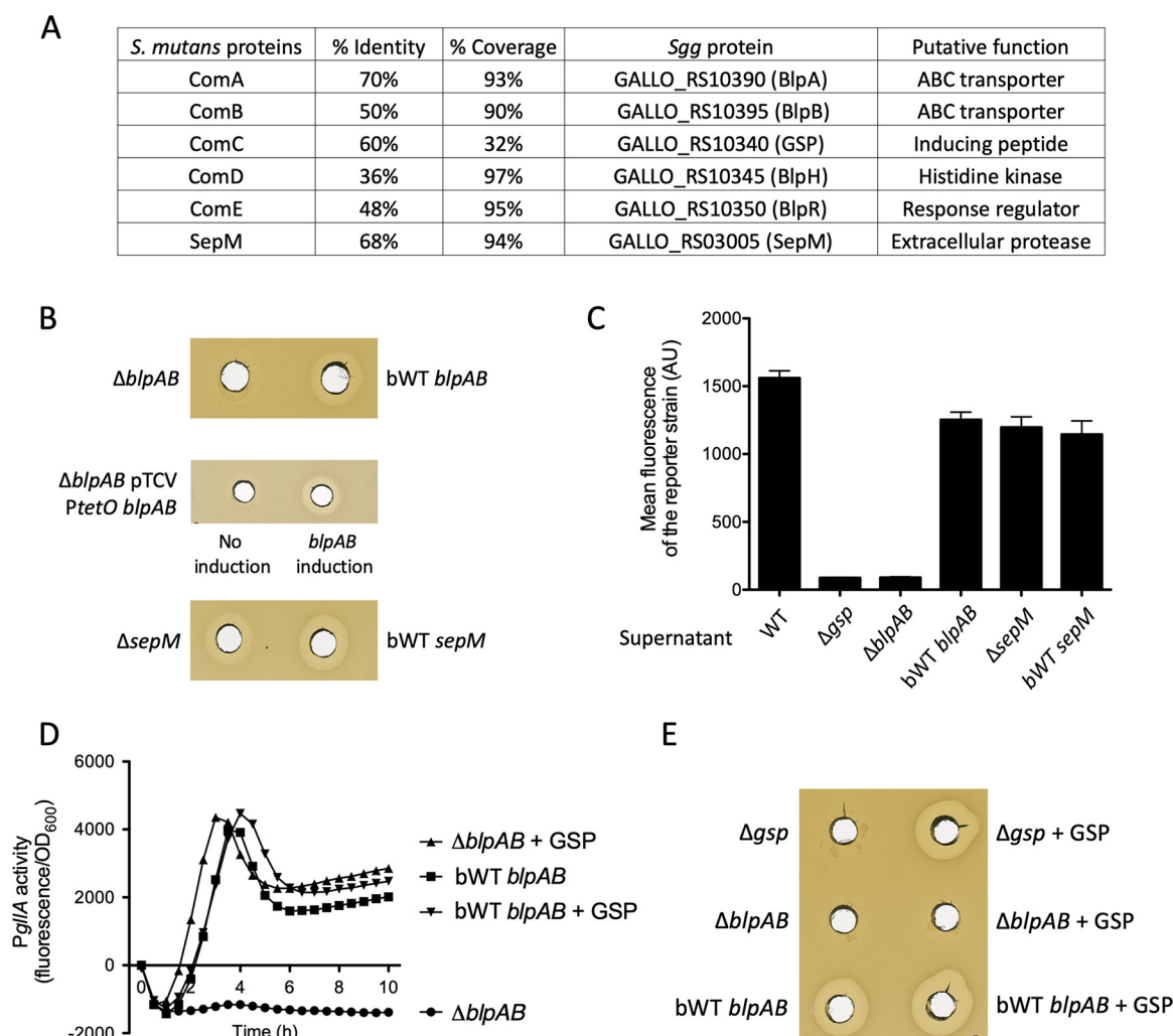
FIG 1 The ABC transporter BlpAB secretes both GSP and gallicin peptides. (A) Summary table of BLAST results comparing the ComABCDE system and SepM proteins of S. mutans with their homologous counterparts in S. gallolyticus subsp. gallolyticus . (B) Agar diffusion assay showing gallicin activity in the culture supernatant against S. gallolyticus subsp. macedonicus . Strains tested include S. gallolyticus subsp. gallolyticus UCN34 \Delta blpAB and UCN34 \Delta sepM, their bWT counterparts, and complemented S. gallolyticus subsp. gallolyticus UCN34 \Delta blpAB containing the plasmid pTCV \Omega PtetO-blpAB with or without induction of PtetO. (C) Mean fluorescence of the reporter strain S. gallolyticus subsp. gallolyticus UCN34 \Delta gsp pTCV \Omega PgIIA-gfp resuspended in the supernatant of S. gallolyticus subsp. gallolyticus UCN34 WT, \Delta gsp, \Delta blpAB, bWT blpAB, \Delta sepM, and bWT sepM strains. Results are means and standard deviations (SD) from three independent experiments. (D) PgIIA activity in S. gallolyticus subsp. gallolyticus UCN34 \Delta blpAB and its bWT counterpart containing the reporter plasmid pTCV \Omega PgIIA-gfp with or without addition of 20 nM synthetic GSP. One representative curve of three independent experiments is shown here for each condition. (E) Agar diffusion assay showing gallicin activity in the culture supernatant against S. gallolyticus subsp. macedonicus . Strains tested include S. gallolyticus subsp. gallolyticus UCN34 \Delta gsp, \Delta blpAB and bWT blpAB cultivated with or without addition of 20 nM synthetic GSP.
