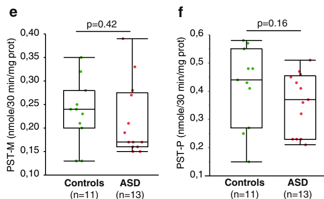
Fig. 2 Phenol sulfotransferase activities in blood, post-mortem pineal glands, and ileal samples from patients with ASD. a–c Blood samples were taken in the morning from 97 unrelated individuals with ASD, their first-degree relatives (138 parents and 56 unaffected sibs), and 106 controls. a Platelet PST-M activities, b Platelet PST-P activities, c , d Pineal gland samples were obtained from 9 patients with ASD and 22 age- and sex-matched controls. e , f Ileal samples were obtained from 13 patients with ASD and 11 matched controls. Boxes indicate medians and quartiles. Dashed lines indicate the threshold of the 5th percentiles of the control group. Groups were compared using the Wilcoxon two-sample test.
