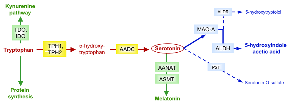
Fig. 1 Serotonin metabolism. Serotonin is synthesized from tryptophan (red steps) by tryptophan hydroxylases (TPH1, non-neuronal, and TPH2, neuronal) and aromatic amino-acids decarboxylase (AADC). Of the two catabolic pathways (blue steps), the major one sequentially involves monoamine oxidase A (MAO-A) and aldehyde dehydrogenase (ALDH) or reductase (ALDR). Sulfoconjugation by phenol sulfotransferases (PST) is a quantitatively minor pathway. Alternatively, tryptophan can enter the kynurenine pathway after oxidation by indoleamine-2,3-dioxygenase (IDO) or tryptophan 2,3-dioxygenase (TDO), or serotonin be converted into melatonin by arylalkylamine N-acetyltransferase (AANAT) and acetylserotonin methyltransferase (ASMT).
