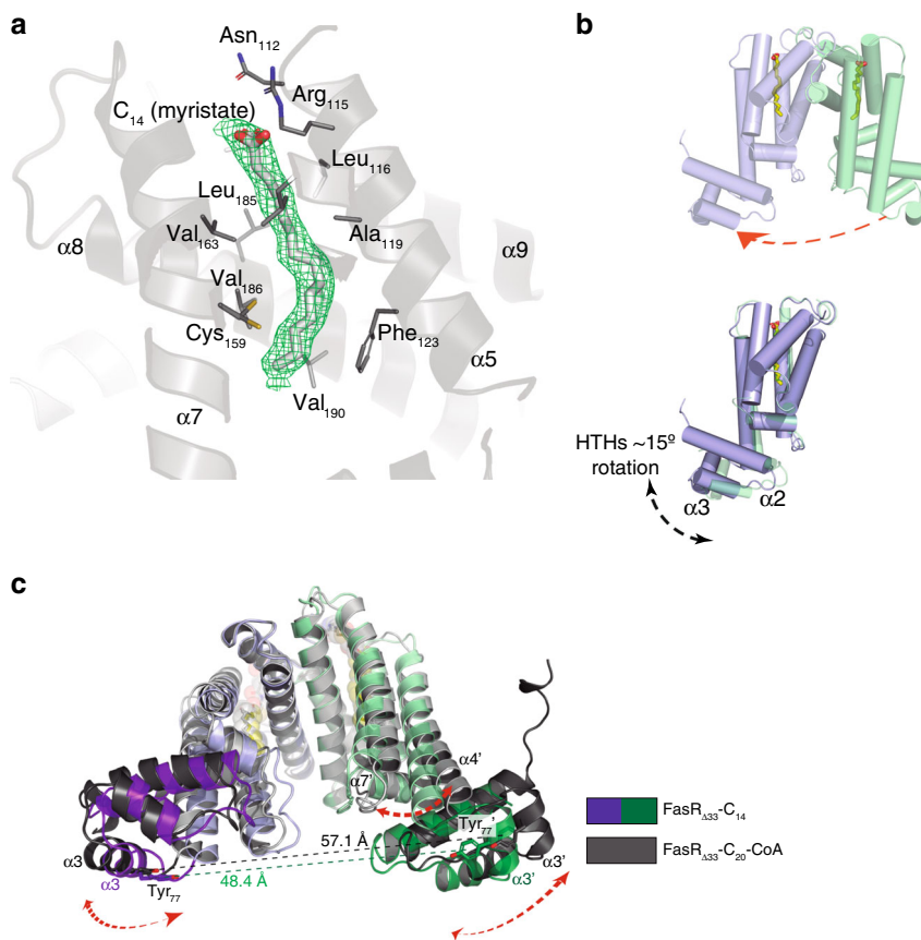
Fig. 2 FasR \Delta_{33} -C _{14} exhibits larger protein flexibility including dimer asymmetry. a SigmaA-weighted mF_{obs}-DF_{calc} difference Fourier map contoured at 3.5\sigma (green mesh) calculated with no ligand bound in the effector-binding tunnel during FasR \Delta_{33} -C _{14} refinement. The FasR \Delta_{33} -C _{14} model is shown with grey cartoons, and residues at \leq 4 Å from the ligand are depicted with thin sticks. The electron density allowed to model a myristic acid, overlaid within the difference map in thick sticks coloured by atom. Note polar and charged residues on the top opening, close to the carboxyl head of the ligand. Hydrophobic residues line up the rest of the tunnel's walls. b FasR \Delta_{33} -C _{14} protomers A and B are coloured as in Fig. 1. The dimer is asymmetric, quantitated by superimposing protomer B onto A (red arrow in the top panel), after what the effector-binding domains fit quite well while the HTH domains show significant rotation between one another (bottom panel), with max root-mean-square deviation (rmsd) on helices \alpha 2 and \alpha 3 . c The FasR \Delta_{33} -C _{20} -CoA and FasR \Delta_{33} -C _{14} structures are superposed, resulting in maximal fit on the central 4-helix bundle that mediates dimerisation (helices \alpha 8 - \alpha 9 from both protomers). The upper portion of the effector-binding domains end up well aligned, but significant shifts affect the lower part together and the HTH domains (dashed arrows). The distance between the centres of mass of Tyr _{77} on helix \alpha 3 , differs by more than 10 Å between both structures. The HTH domains move consolidated with the bottom portion of juxtaposed helices \alpha 4 and \alpha 7 from the effector-binding domains.
