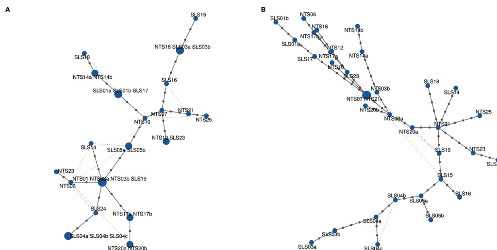
Fig. 2. A: MLST Haplotype network inferred with concatenated sequences data of the nucleotide polymorphic sites at the four loci (ITS1, mt26S, SOD and CYB). Fig. 2 B: MLP Haplotype network inferred with amplicon length data of the six microsatellites markers (STR022, STR108, STR138, STR189, STR278, and STR279). Blue circle = Haplotype/Genotype described within the sample (name of the sample, followed by a letter if several genotypes described in this sample). The dots separating two haplotypes correspond to the number of mutational steps needed to relate two distinct haplotypes. SLS: Saint-Louis; NTS: Nantes. (For interpretation of the references to colour in this figure legend, the reader is referred to the web version of this article.)
