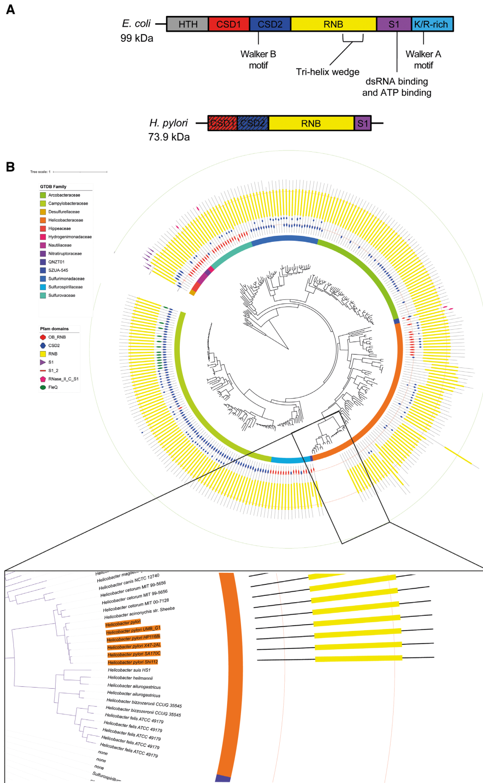
Figure 1. (A) Schematic representation of the functional domain organization of E. coli RNase R ( EcRNaseR ) and H. pylori RNase R ( HpRNase R ). The CSD1 and CSD2 domains of HpRNase are hatched to illustrate the poor conservation of these regions compared with EcRNaseR . (B) Phylogenetic tree illustrating the evolution and conservation of the characteristic domains of RNase R. (For more details, see supplementary Figure S2). The tree species has been pruned to preserve only strains with full-sized proteins, while retaining strains of the genus Helicobacter E from GTDB that do not code for RNase R. The names of strains of the H. pylori species are highlighted in orange. The GTDB Taxonomy Family Rank has been used as a color code. The location of the pfam profiles predicted with hmmscan is reported on the sequences represented by black lines. Note that the first cold-shock domain (CSD1) can also be annotated OB_RNB or CSD2 in Pfam profiles. Details of the data for the Helicobacteraceae family are magnified on the bottom part of the figure. The figure was obtained with the iTOL v5 software ( https://itol.embl.de ).
