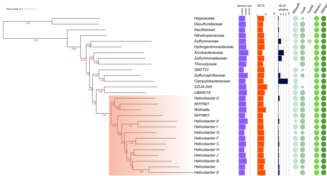
Figure 7. Taxonomic distribution of the protein families of RNases, RNase R, RNase J and PNPase and of the CsdA helicase. The phylogenetic tree has been pruned at the family rank except for the Helicobacteraceae , where it is at the genus level (orange shading). The average sizes of the genomes and their average G+C content is mentioned, as well as the number of genomes (strains) analyzed per family rank. The diameter of the circles is proportional to the percentage of homologous genes observed in the genomes clustered under each taxonomic rank. CsdAS refers to a group of CsdA paralogues that was found only in the Sulfurovaceae . The figure was made with iTOL v5.
