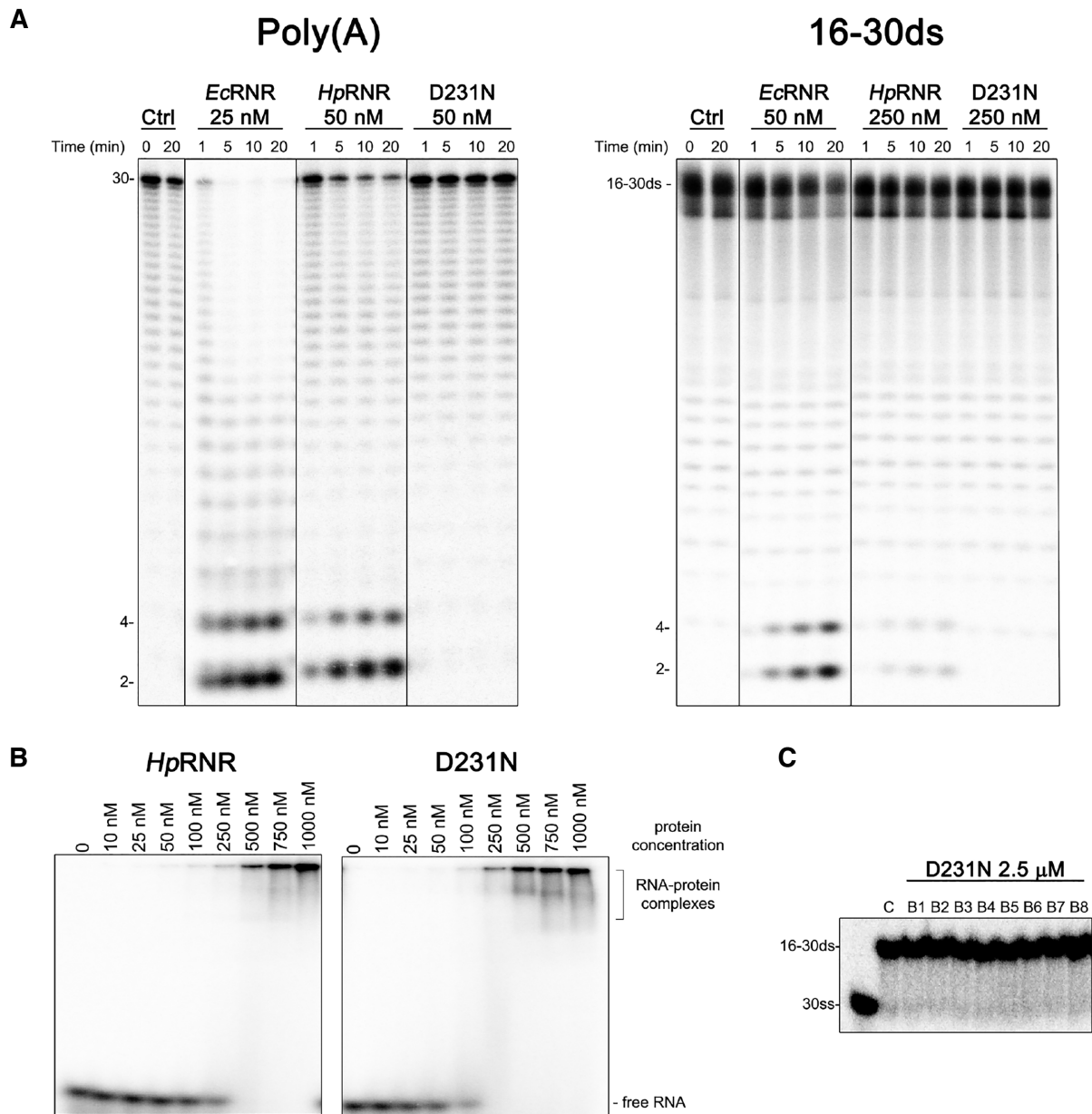
Figure 2. In vitro , Hpr Nase R displays 3'-5' exoribonuclease activity but no helicase activity. (A) 3'-5' exoribonuclease activity tests over 20 min, of Ec RNases R and Hpr Nase R on a poly(A) ssRNA substrate (left panel) or on a 16-30ds partially dsRNA substrate (right panel). The catalytically inactive Hpr Nase R D231N mutant served as a control. The end-products are indicated as we previously reported (79). (B) Electrophoretic mobility shift assay (EMSA) of wild type Hpr Nase R and the Hpr Nase R D231N mutant. (C) Helicase activity assay of the catalytically inactive Hpr Nase R D231N mutant using eight different buffers B1 to B8. B1: 50 mM Tris-HCl pH 7.5, 5 mM ATP, 50 mM MgCl 2 , and 20 mM NaCl; B2: 50 mM Tris-HCl pH 7.5, 5 mM ATP, 5 mM MgCl 2 and 50 mM NaCl; B3: 20 mM Tris-HCl pH 7.5, 5 mM ATP, 5 mM MgCl 2 and 75 mM NaCl; B4: 20 mM Tris-HCl pH 7.5, 5 mM ATP, 5 mM MgCl 2 , 75 mM NaCl and 1 mM DTT; B5: 10 mM HEPES pH 7.4, 5 mM ATP, 5 mM MgCl 2 , 75 mM NaCl and 1 mM DTT; B6: 10 mM HEPES pH 7.4, 5 mM ATP, 5 mM MgCl 2 and 75 mM NaCl; B7: 20 mM HEPES pH 7.4, 5 mM ATP, 5 mM MgCl 2 , 75 mM NaCl and 1 mM DTT; B8: 10 mM HEPES pH 7.4, 5 mM ATP, 5 mM MgCl 2 , 50 mM NaCl and 1 mM DTT.
