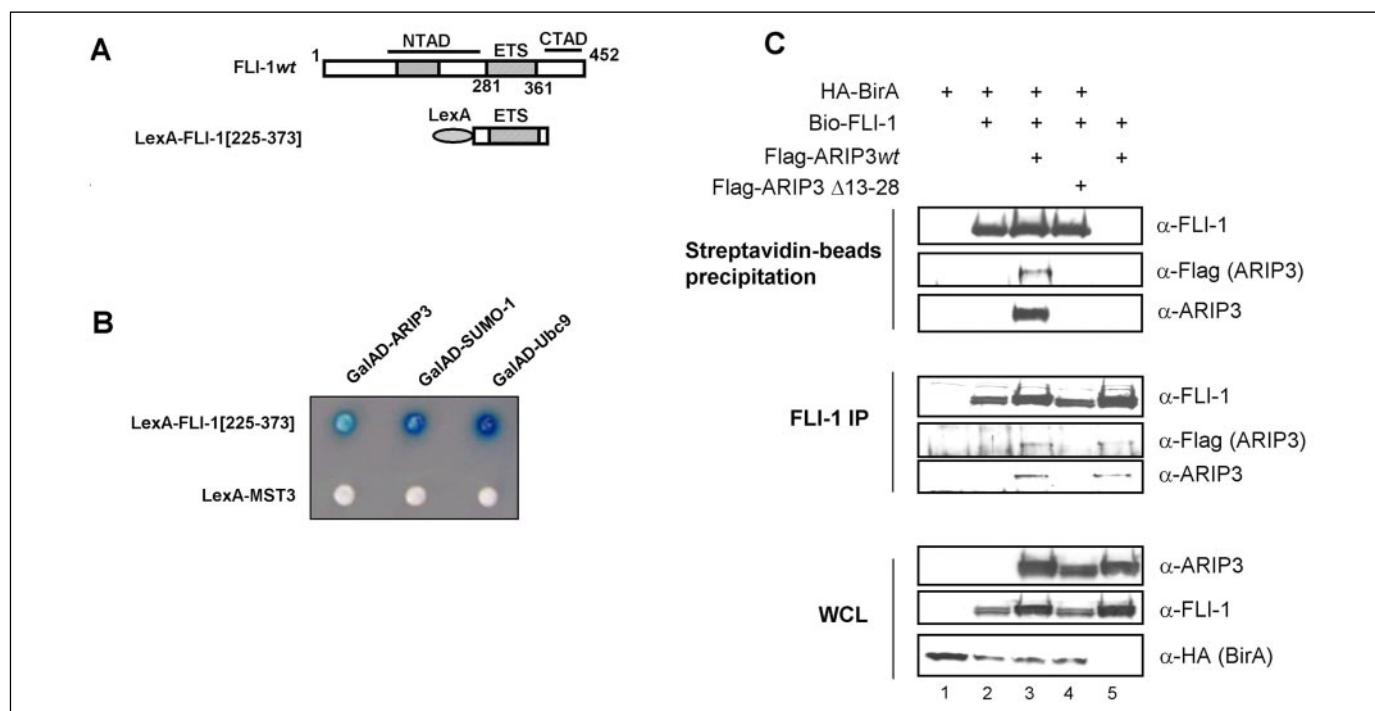
FIGURE 1. Schematic diagram of the FLI-1 protein and the interaction of FLI-1 and PIASxα. A , shown is a diagram of the FLI-1 functional domains. The ETS domain is shown as a hatched box, and the pointed/SAM domain as a gray box. NTAD, N-terminal activation domain; CTAD, C-terminal activation domain. The LexA fusion protein encompassing amino acids 225–373 of FLI-1, used as bait in the yeast two-hybrid screen, is depicted. LexA-MST3 (full-length) was used as a negative control. B , transformants were assayed for \beta -galactosidase activity and analyzed by LacZ staining. C , 293 cells were transfected with combinations of expression plasmids encoding the indicated proteins. Biotagged FLI-1 (Bio-FLI-1) was isolated by affinity chromatography using streptavidin beads (upper panels) or by immunoprecipitation (IP) using anti-FLI-1 antibody (middle panels) as described under “Experimental Procedures,” and blots were processed for Western analyses using anti-FLAG, anti-ARIP3, or anti-FLI-1 antibody to detect FLAG-ARIP3 and FLI-1. Whole cell lysates (WCL) used in the immunoprecipitation and affinity chromatography analyses were subjected to SDS-PAGE and processed for Western blotting using anti-ARIP3, anti-FLI-1, or anti-HA antibody to confirm expression and input of the respective proteins (lower panels).
