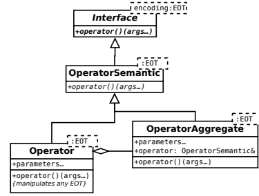
Figure 1: UML diagram of a high-level view of the main design pattern used in the Paradiseo framework.
