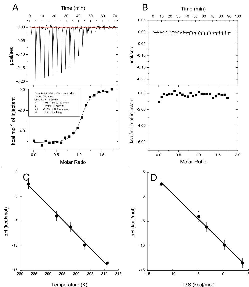
Figure S3: (A) Isothermal titration calorimetry of CaM by P454 in buffer B at 25°C using a VP-ITC instrument. Titration was performed by injections of 13 μL of P454 (loaded in the syringe at 90 μM) into the cell containing CaM at 10 μM (see Table S3 for ΔG values). (B) Isothermal titration calorimetry of CaM by P454 in buffer A complemented with 0.2 mM EDTA at 25°C. Titration was performed by consecutive injections of 10 μL of P454 (loaded in the syringe at 90 μM) into the cell containing CaM at 10 μM. (C) ITC experiments were performed at various temperatures to infer the heat capacity of the reaction. The slope of \Delta H=f(T) provides us with the heat capacity \Delta C_p of the P454:CaM complex. The \Delta C_p value is negative, as measured for canonical CaM-binding peptides 36 , however, lower than those measured for globular peptide:CaM complexes, suggesting that the P454:CaM complex does not adopt a globular conformation. This is confirmed by X-ray and SAXS data reported in this article. (D) Representation of the enthalpy-entropy compensation (EEC) plot derived from ITC experiments of P454:CaM titrations at different temperatures. The P454:CaM complex formation at various temperatures follows a typical entropy-enthalpy compensation. The enthalpy and temperature values are listed in Table S2. S.D for ΔH values is ± 1 kcal/mol.
