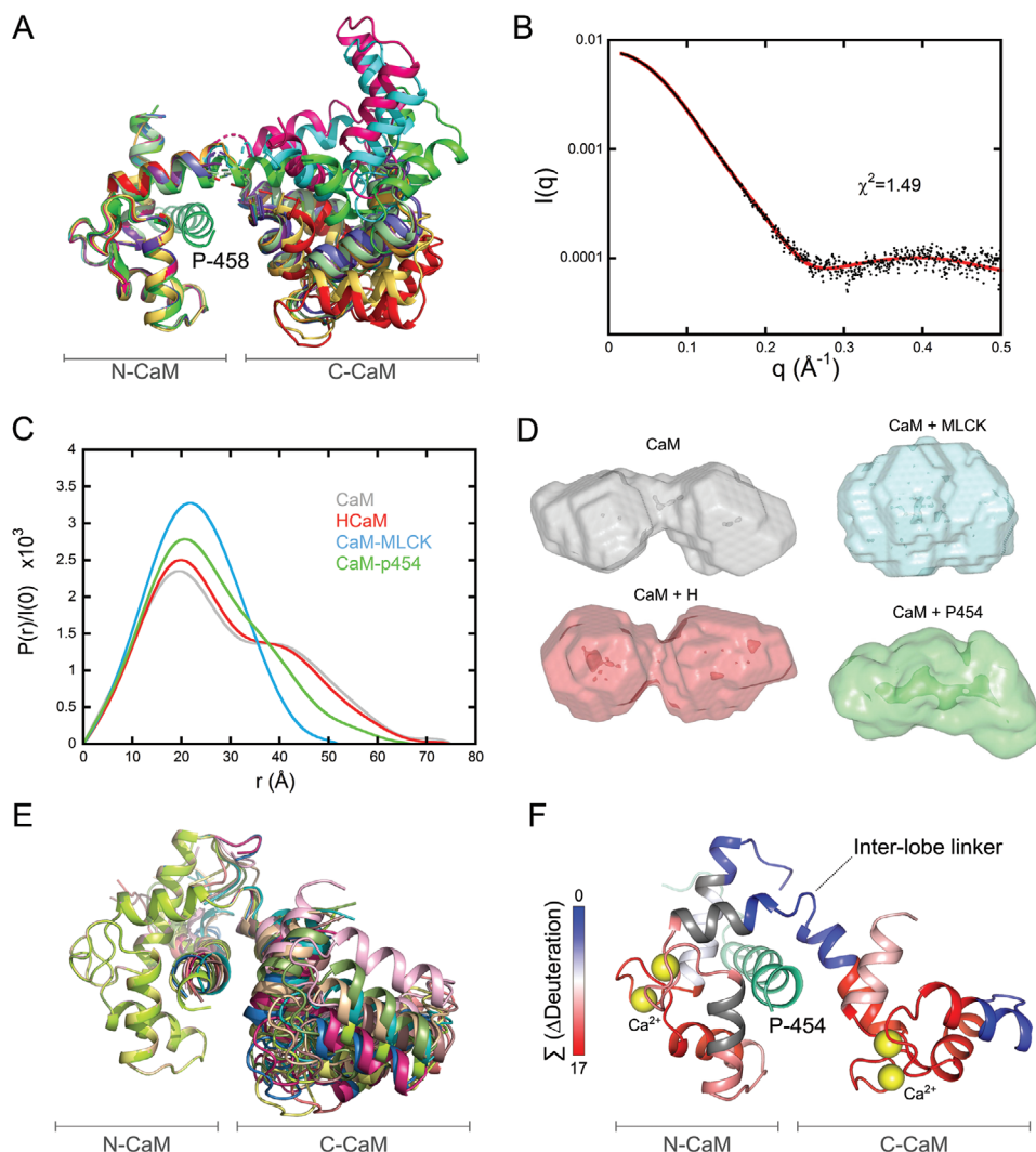
Figure 2. Structure and dynamics of the P454:CaM complex. A) The twelve P458:CaM crystal structures (PDB 6YNS) are displayed after superimposition of C_\alpha s over the range 10 to 70 included, corresponding to the N-ter lobe of calmodulin. The crystal structure 1CLL [92] of the extended conformation of CaM is shown in light green. B) Experimental SAXS curve of the P454:CaM complex (black dots) superimposed over the best fit (red curve) obtained from the structural model shown in Figure 2F. C) Comparison of the four distance distribution functions obtained using the program GNOM for CaM alone (grey), H:CaM (red), MLCK:CaM (cyan), and P454:CaM (green) complexes. D) DAMMIN models of CaM alone, H:CaM, MLCK:CaM, and P454:CaM complexes, shown with the same color code. E) Ten models fitting the SAXS curve shown on Figure 2B obtained using the program DADIMODO [68] are displayed after superimposition of C_\alpha s over the range 10 to 70. F) Effects of P454 on the HDX behavior of CaM. The uptake differences ( \Delta Deuteriation) measured between the free- and P454-bound CaM were extracted for each peptide at each time point, summed, and plotted on the best-fitting structural model of P454:CaM (red curve in 2B). The summed \Delta Deuteriation values [ \Sigma ( \Delta Deuteriation)] are colored from blue (no variation of deuterium uptake) to red (major reductions of deuterium uptake). Uncovered regions are in grey.
