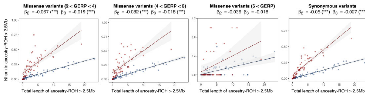
FIG. 4. Fraction of N_{hom} in ancestry-specific ROHs versus the total length of ancestry-specific ROHs per individual. South Asian ROHs in red, and European ROHs in blue. The first three panels show a deleterious GERP category each and the last panel shows synonymous variants. \beta_2 and \beta_3 show intercept and slope differences between regressions. * P value < 0.05; ** P value < 0.01; *** P value < 0.001.
