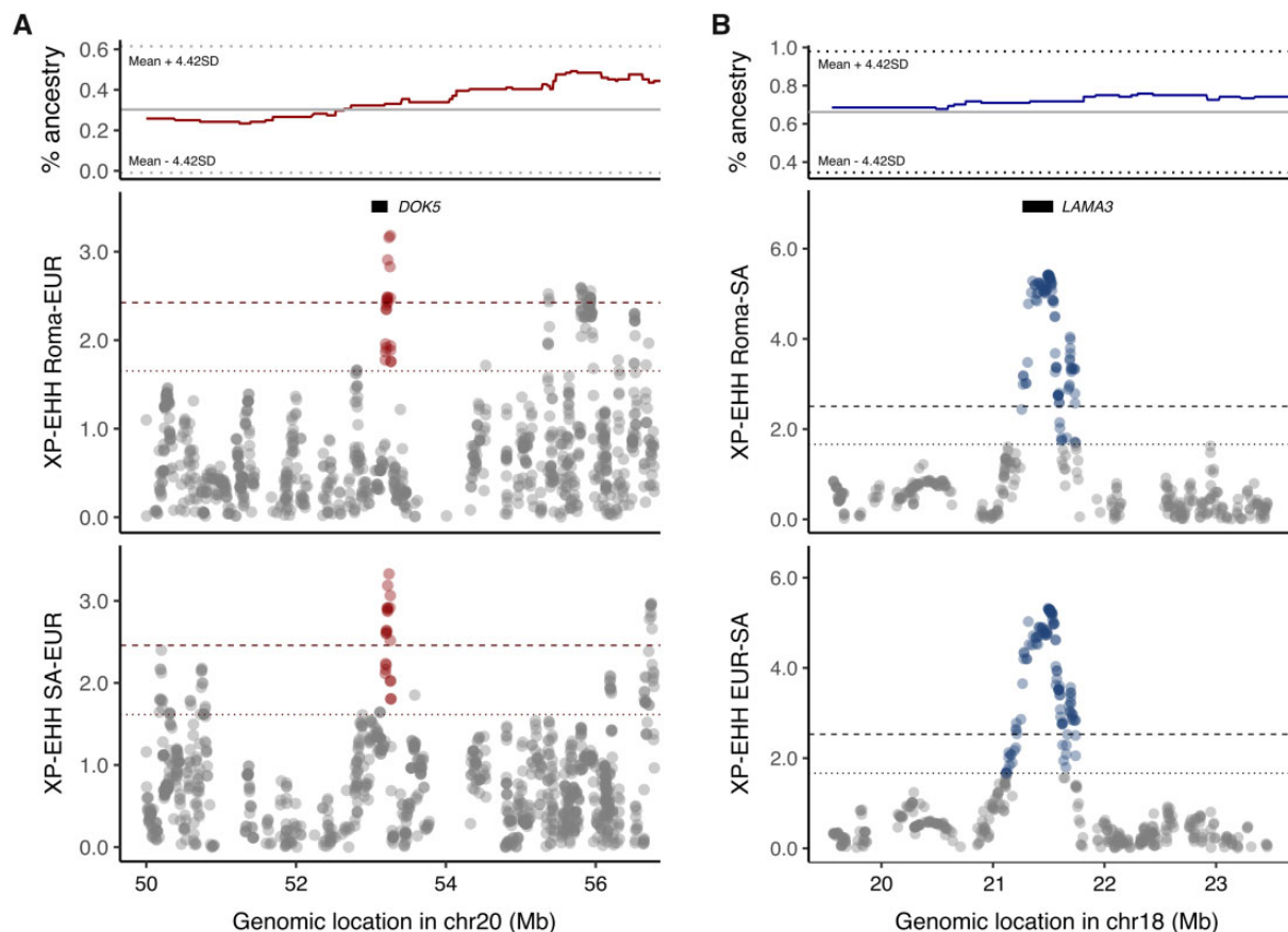
FIG. 5. Selection tests results (XP-EHH) and mean local ancestry in two candidate regions. (A) Results for chromosome 20: 50,000,000–56,000,000. Top panel shows South Asian (dark red) ancestry (mean and 4.42 standard deviations in solid and dotted lines, respectively). Genomic location of DOK5 gene is shown. Middle and bottom panels show XP-EHH analysis comparing Roma against Europe and South Asia against Europe (top 1% and 5% are shown with dashed lines). The region within chr20: 52,813,832–53,454,024 is highlighted in red. (B) Results for chromosome 18: 20,000,000–23,000,000. Top panel shows European (blue) ancestry (mean and 4.42 standard deviations in solid and dotted lines, respectively). The genomic location of LAMA3 gene is shown. Middle and bottom panels show XP-EHH analysis comparing Roma against South Asia and Europe against South Asia (top 1% and 5% are shown with dashed lines). The region within chr18: 21,276,048–21,740,878 is highlighted in blue.
