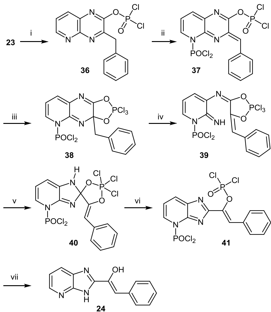
Scheme 4 Suggested mechanism for the rearrangement of 23 into 24 . i: 1st addition of \text{POCl}_3 , (- HCl). ii: 2nd addition of \text{POCl}_3 , (- HCl). iii: cyclisation (+ HCl). iv and v: rearrangement of the carbon-nitrogen bond. vi: HCl elimination. vii: hydrolysis (upon treatment) of the two phosphoryl dichlorides.
