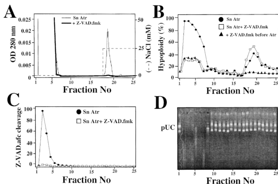
Figure 3. Selective retention of AIF activity on a MiniS cation exchange column. (A) Interference pattern showing OD 280 nm (solid line) and NaCl concentration (dashed line) versus Fraction No. (1 to 25). (B) Profile of AIF activity (Hypoploidy %) versus Fraction No. (1 to 25) for Sn Atr (filled circles), Sn Atr + Z-VAD.fmk (open squares), and + Z-VAD.fmk before Atr (filled triangles). (C) Z-VADase activity (Z-VAD.afc cleavage) versus Fraction No. (1 to 25) for Sn Atr (filled circles) and Sn Atr + Z-VAD.fmk (open squares). (D) Gel electrophoresis image showing DNase activity (pUC) versus Fraction No. (1 to 25). Results are representative of ten independent experiments.
