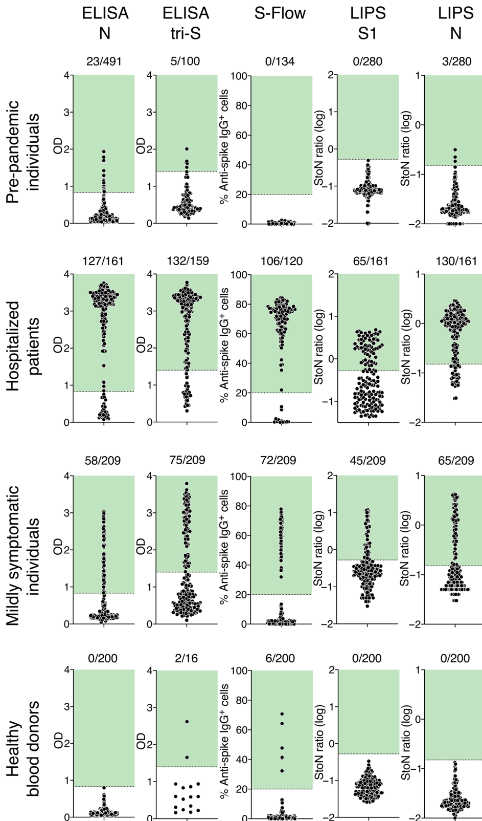
Fig. 1. Serological survey of SARS-Cov-2 antibodies in human serum samples. Four serological assays were used to detect anti-SARS-Cov-2 antibodies in serum samples: (top row) individuals sampled between 2017 and 2019 (before pandemic), (second row) hospitalized cases with confirmed COVID-19, (third row) mildly symptomatic individuals from the Crépy-en-Vallois pandemic cluster with suspected COVID-19, and (bottom row) healthy blood donors. ELISA N and ELISA tri-S assays are conventional ELISAs using either N protein or the trimeric ectodomain of S protein as antigens. S-Flow is an assay detecting antibodies bound to cells expressing S protein by flow cytometry. The LIPS S1 and N assays detect either S1 or N protein fused to luciferase by immunoprecipitation. Pre-pandemic serum samples were used to determine the cutoff for each assay, which is indicated by a dotted line and a green area. The two ELISA assays were set to 95% specificity; the specificity of the S-Flow assay and LIPS assay was 99%. The number of positive samples is indicated. Each dot represents one sample. OD, optical density; StoN, signal-to-noise ratio.
