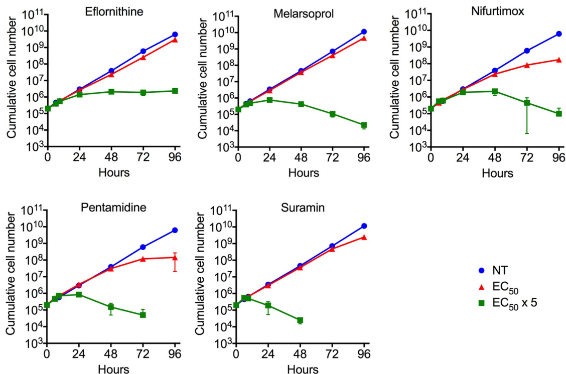
Fig 1. T. brucei growth profiles during exposure to antitrypanosomal drugs. Parasites were treated with each of the five clinical antitrypanosomal at 1 x EC_{50} and 5 x EC_{50} concentration. Cells that are not treated (NT) are shown as controls. Data are averages of four technical replicates. Error bars show standard deviation.
