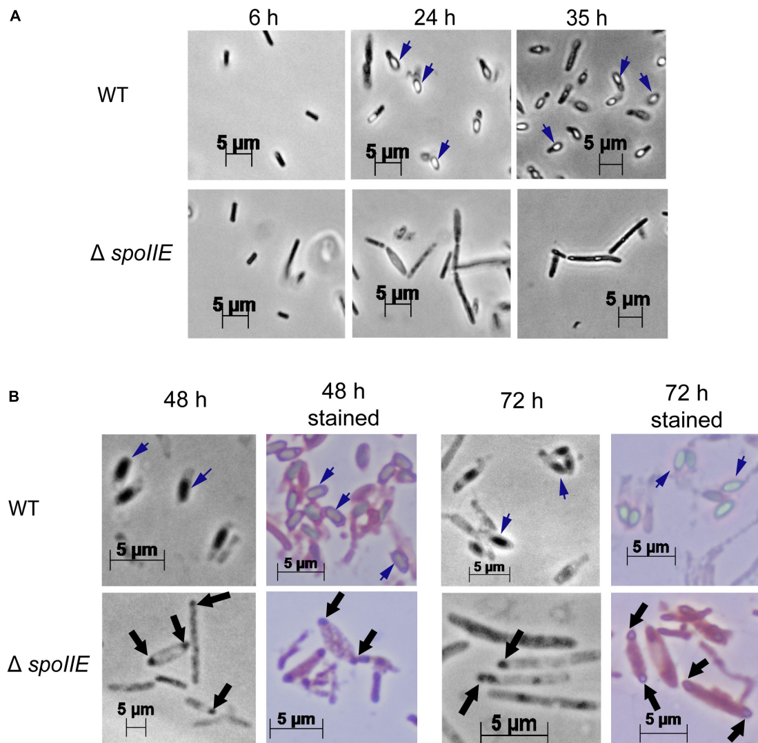
FIGURE 4 | Phase-contrast microscopy images of C. beijerinckii WT and \Delta spoIIE cells during the fermentation. While mature spores were seen in the WT images after 24 h of cultivation, no spores were seen in \Delta spoIIE cultures even after 72 h of cultivation. However phase-dark bodies, stained in blue by Shaeffer-Fulton staining, were observed in the \Delta spoIIE cells after 48 h of cultivation (A) Pictures with x400 magnification at 6 h, 24 h and 35 h; (B) Pictures at 48 h and 72 h of culture with x1000 magnification with and without Shaeffer-Fulton stain. The short dark blue arrows indicate mature spores. The black arrows indicate the phase-dark masses at the poles of the mutant cells.
