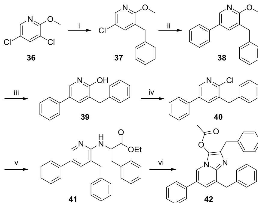
Scheme 5. i: \text{PhCH}_2\text{ZnBr} , \text{Pd}(\text{OAc})_2 , XPhos, THF, 60 °C. ii: \text{PhB}(\text{OH})_2 , \text{Pd}(\text{OAc})_2 , SPhos, dioxane/ \text{H}_2\text{O} 5:1, 90 °C. iii: 33% \text{HBr}/\text{AcOH} , 100 °C. iv: \text{PhPOCl}_2 , 150 °C. vi: PheOEt ( 23 ), \text{Pd}(\text{OAc})_2 , BINAP, \text{Cs}_2\text{CO}_3 , toluene, 90 °C. vii: 1) \text{NaOH} , THF, 20 °C, 2) \text{Ac}_2\text{O} , 20 °C.
