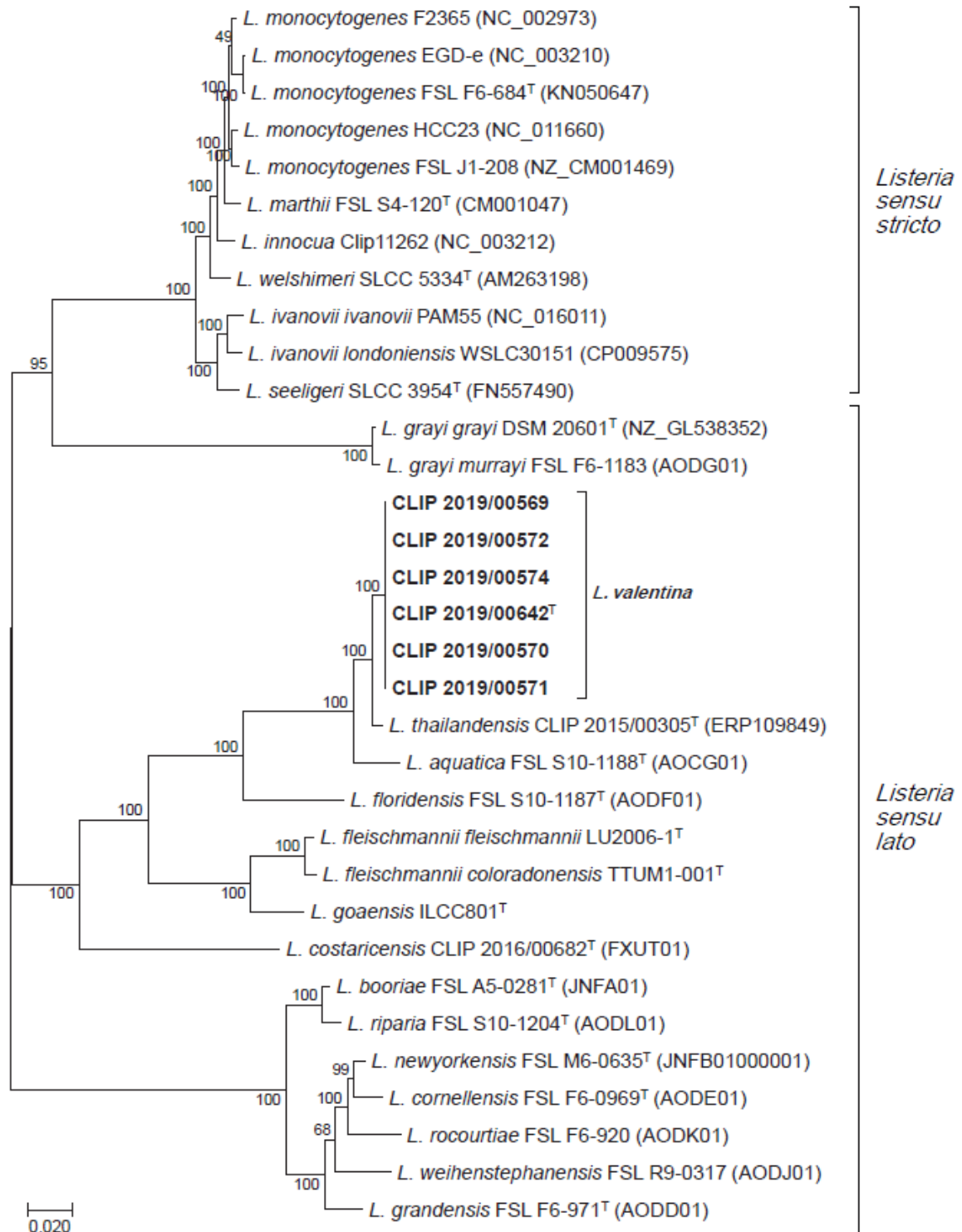
FIGURE 2. Maximum likelihood phylogenetic analysis based on the concatenated amino acid sequences of 231 core genes present in all Listeria species. Distance estimation was obtained by the Whelan and Goldman (WAG) model [38]. Branch lengths represent the number of amino acid substitutions per site and bootstrap percentages of 1,000 replicates are shown. GenBank accession numbers are provided in brackets. Listeria valentina isolates are highlighted in bold.
