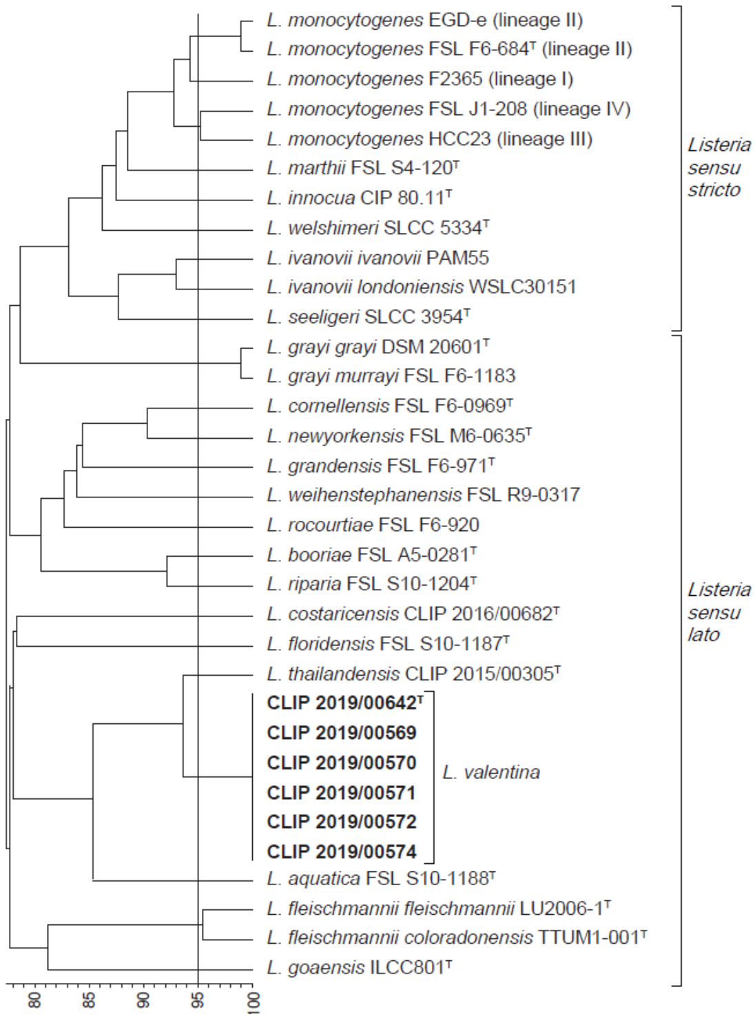
FIGURE 3. UPGMA clustering based on the genomic average nucleotide difference (ANI). The vertical dashed bar represents the proposed 95% ANIb species cut-off that correlates with the 70% DNA-DNA hybridization threshold [43]. Scale bar represents the percentage of similarity. Listeria valentina type strain is highlighted in bold.
