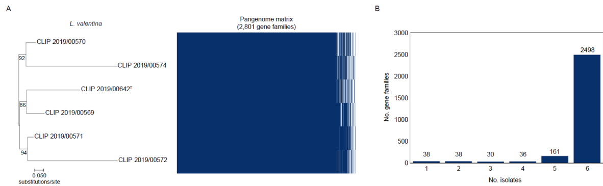
Supplementary Figure 1. Pangenome analysis of L. valentina sp. nov. isolates. A) Presence (blue) and absence (white) patterns of the 2,801 gene families in each isolate, as determined by Roary (Page et al. , 2015), using a 95% BLASTP identity cut-off. A midpoint rooted recombination-free phylogeny built from the L. valentina genome alignment (2,536,866 nucleotide positions) using Parsnp (Treangen et al. , 2014) is shown on the left. Numbers at the nodes indicate the bootstrap values based on 1,000 replicates. B) Frequency plot of the gene families versus the number of isolates.
