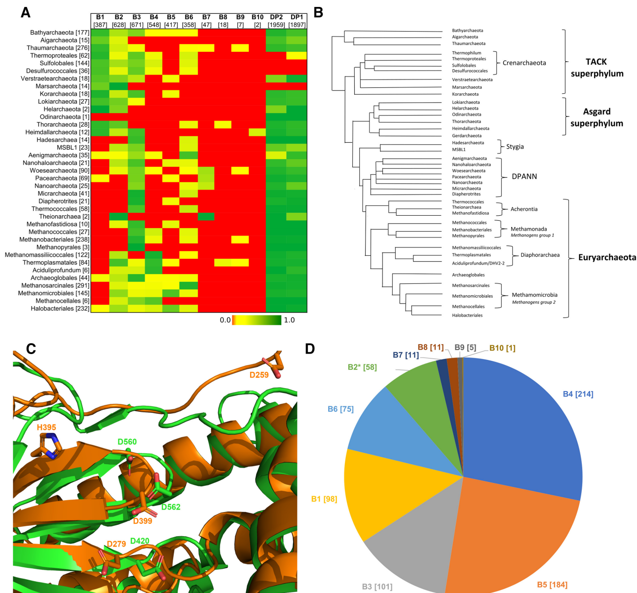
Figure 5. Archaeal PolBs. (A) Distribution of PolBs, PolD large (DP2) and small (DP1) subunits in archaeal genomes taken from GenBank (Supplementary Table S4). Numbers of species in a taxon and groups are shown in brackets. (B) The unrooted evolutionary tree of Archaea which is based on the schematic tree (70) updated according to recent phylogenetic analyses (49,71,72). (C) Model of B2 PolB (AAK41686) from Saccharolobus solfataricus P2 active site (orange) aligned to PolB3 from Pyrobaculum calidifontis (green color, PDB:5mdn). (D) B2 group members are often found together with other archaeal PolBs in the same organism. Co-occurrences are represented as a pie chart. Total of 628 genomes encode B2, 58 of them have B2 as a sole PolB (marked with an asterisk).
