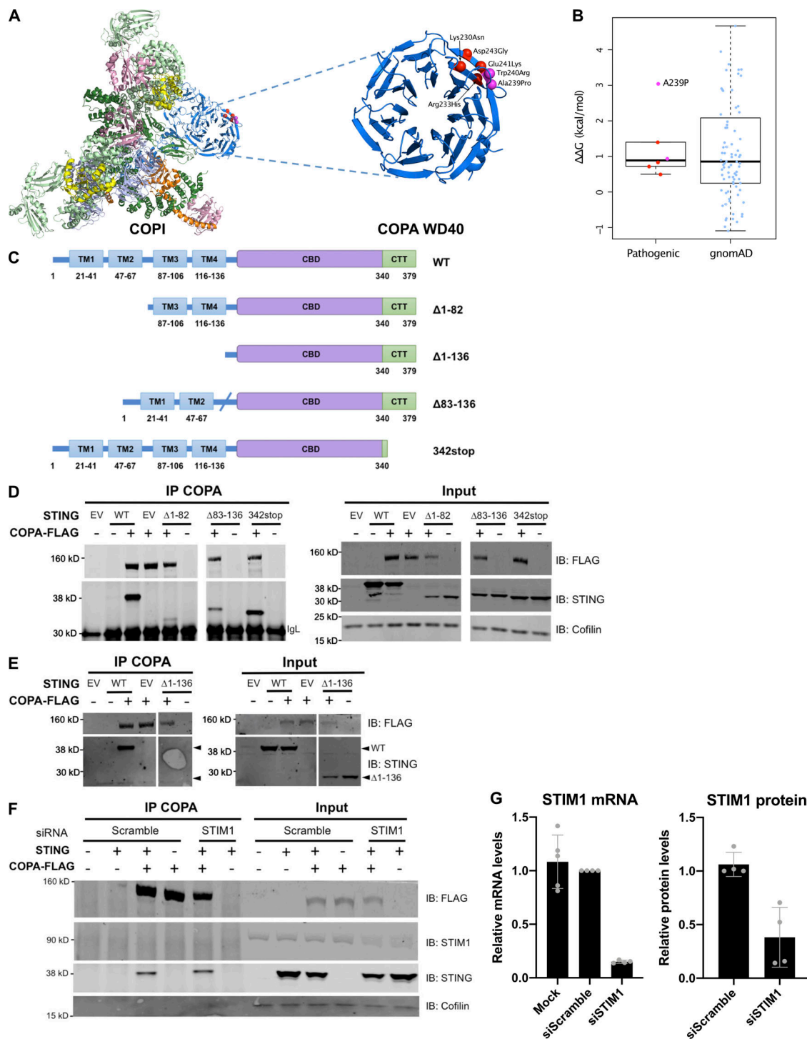
Figure S3. COP1 complex and physical interaction of COPA and STING. (A) Location of pathogenic COPA mutations within the structure of the COP1 coat leaf (PDB ID: 5NZR). The four mutations from this study are shown in red, and two previously reported mutations are shown in magenta. (B) Predicted effects of pathogenic mutations and putatively benign substitutions present in the gnomAD database on protein stability, calculated with FoldX. (C) Schematic representation of WT STING and truncated STING plasmids (i.e., \Delta 1-82 , \Delta 83-136 , \Delta 1-136 , and 342stop). (D) Western blot analysis of FLAG, STING, and Cofilin in proteins IP with an antibody against FLAG (IP COPA), and whole-cell lysates (input) of HEK293T cells cotransfected with EV (EV or –), or WT COPA and WT STING, or truncated STING plasmids, i.e., \Delta 1-82 , \Delta 83-136 , and 342stop (data representative of three independent experiments). (E) Western blot analysis as in F of proteins IP with an antibody against FLAG (IP COPA), and whole-cell lysates (input) of HEK293T cells cotransfected with EV (EV or –), or WT COPA and WT STING, STING \Delta 1-136 (data representative of two independent experiments). (F) Western blot analysis of FLAG, STING, STIM1, and Cofilin in proteins IP with an antibody against FLAG and in whole-cell lysates (input) of HEK293T cells cotransfected with EV (–) or WT STING and WT COPA plasmids and with a scrambled siRNA or a siRNA pool targeting STIM1. Results are representative of three independent experiments. (G) Quantification of STIM1 silencing assessed by mRNA (left) and protein (right) levels measured, respectively, by RT-qPCR and Western blot 72 h after transfection. Error bars represent SDs. Results are representative of three independent experiments. CTT, C-terminal tail.
