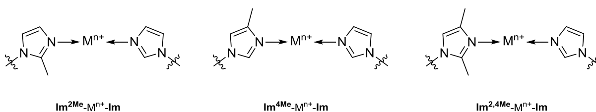
Fig. 4. Chemical structures of dIm 2Me -M n+ -dIm , dIm 4Me -M n+ -dIm and dIm 2,4Me -M n+ -dIm .
