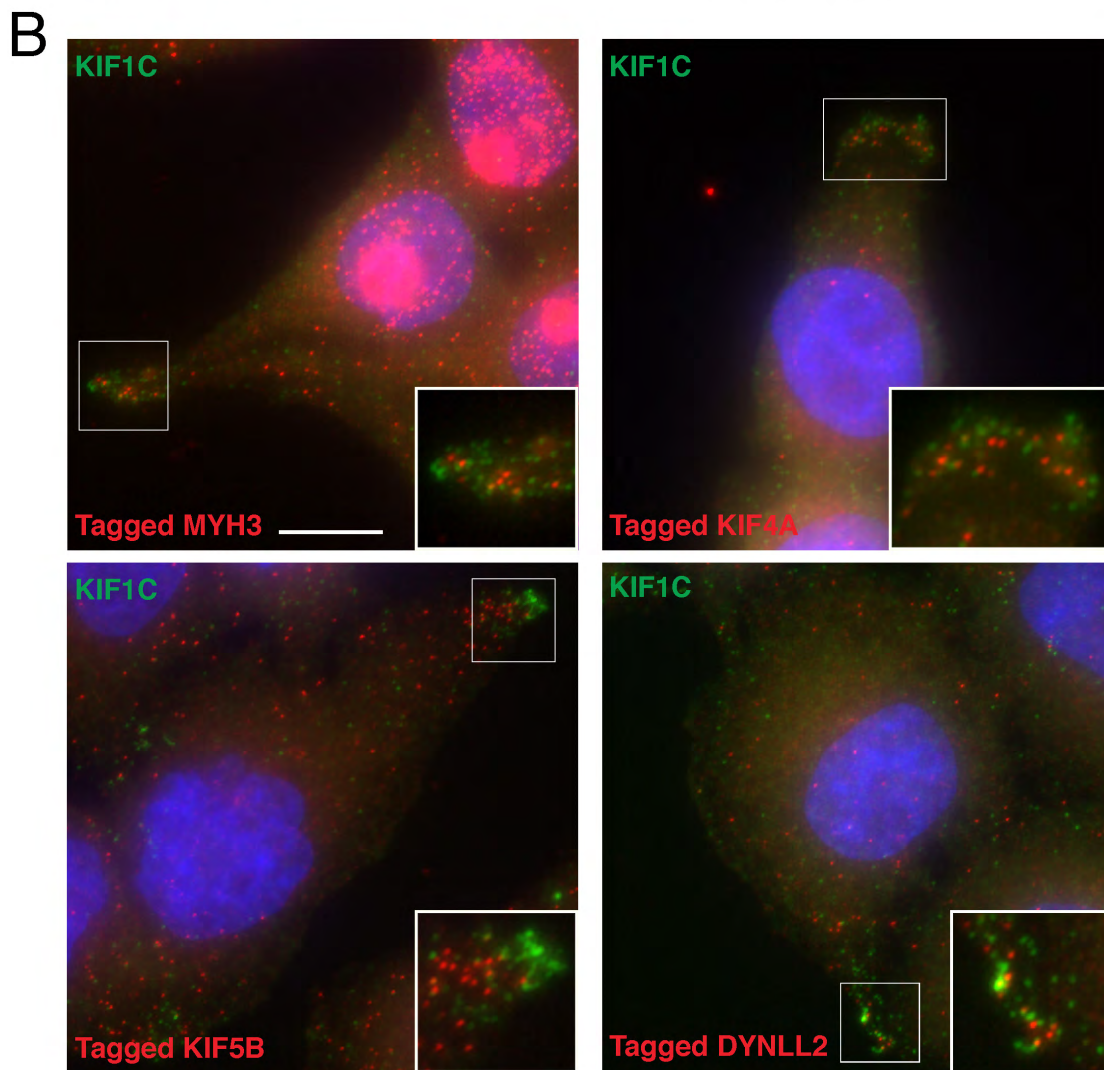
Figure S3, related to Figure 1. Localization of mRNAs in cytoplasmic protrusions.
