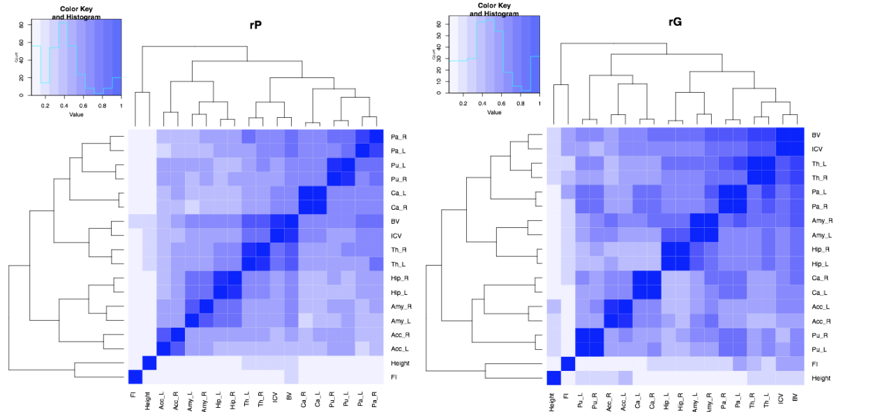
Figure S7. Heat maps of phenotypic correlations ( r_p , left panel) and genetic correlation ( r_g , right panel) values computed with GCTA. The following phenotypes are represented: the left and right hemisphere volumes of accumbens (Acc_L and Acc_R), amygdala (Amy_L and Amy_R), caudate (Cau_L and Cau_R), hippocampus (Hip_L and Hip_R), pallidum (Pa_L and Pa_R), putamen (Pu_L and Pu_R), and thalamus (Th_L and Th_R) ; brain volume (BV), intracranial volume (ICV), height and fluid intelligence (FI) are also represented. Ward hierarchical clustering based on euclidean distance was used to cluster the phenotypes.
