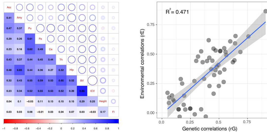
Figure S8. Left: values of environmental correlations are shown in the lower triangular part of the matrix. Circles's diameter is proportional to the strength of the correlation, and a thickness proportional to the size of the confidence interval. Right: scatter plot of environmental versus genetic correlations. Genetic and environmental correlations were adjusted for age, center, sex, and the top 10 principal components of the genetic relationship matrix.
