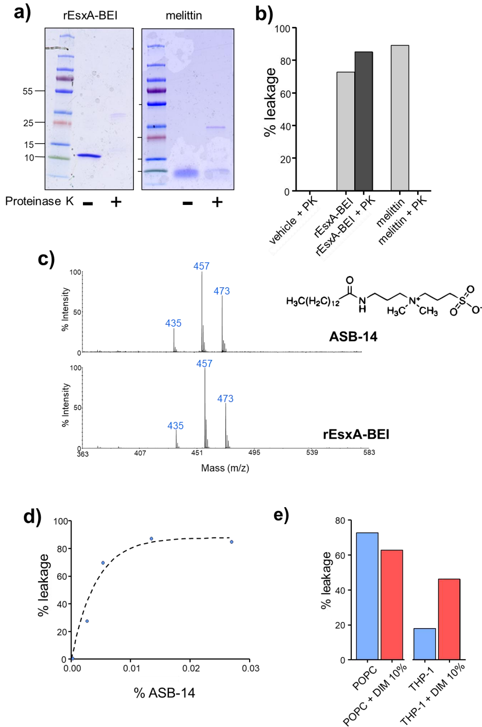
Figure S3. The detergent ASB-14 is detected in rEsxA-BEI samples and exerts a membranolytic activity that can be modulated by DIM. (a) 10 \mu g of rEsxA from BEI (Reference standard, NR-14868) and melittin were digested by Proteinase K for 1h at 37°C. The digestion was verified by SDS-PAGE and Coomassie Blue staining. (b) The activity of intact or digested rEsxA-BEI (10 \mu M) and melittin (50 nM) was tested on POPC liposomes at pH7. (c) 2.5 \mu g of ASB-14 and 1 \mu g of rEsxA-BEI were analyzed by MALDI-TOF mass spectrometry. The mass spectrum shows three peaks representing ASB-14 ions at 435 Da ( M+H^+ ) and pseudomolecular ion ( M+Na^+ ) and ( M+K^+ ) at 457 Da and 473 Da respectively. (d) The membranolytic activity of ASB-14
