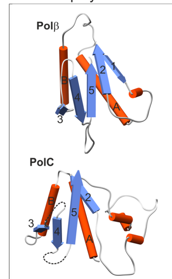
Fig. 1. The core catalytic domains of DNA and RNA polymerases. a Double-psi beta-barrel (DPBB) polymerases. RNAP, multisubunit DNA-dependent RNA polymerase from Thermus thermophilus (PDB ID: 1iw7); eRdRP, eukaryotic RNA-dependent RNA polymerase from Neurospora crassa (PDB ID: 2j7n); PolD, DP2 subunit of family D DNA polymerase from Pyrococcus abyssi (PDB ID: 5ijl). b RRM-fold polymerases. RRM, RNA-recognition motif-containing RNA-binding domain of human nucleolin TIAR (PDB ID: 2cqi); RdRP, RNA-dependent RNA polymerase of poliovirus type 1 (PDB ID: 1ra7); PolA, family A DNA polymerase from Thermus aquaticus (PDB ID: 1taq); ssRNAP, single-subunit DNA-dependent RNA polymerase of bacteriophage T7 (PDB ID: 1msw); RT, reverse transcriptase of Moloney murine leukemia virus (PDB ID: 1mml); PolB, family B DNA polymerase from Thermococcus gorgonarius (PDB ID: 1tgo). c PolC-like polymerases. Polβ, DNA polymerase β from Rattus norvegicus (PDB ID: 1bpb); PolC, family C DNA polymerase from Thermus aquaticus (PDB ID: 2hpi). In b and c , the major secondary structure elements forming the core palm domain are indicated with numbers (for β-strands) and capital letters (for α-helices). Dashed lines indicate regions where insertions into the core palm domains have occurred; these have been omitted for visualization purposes
