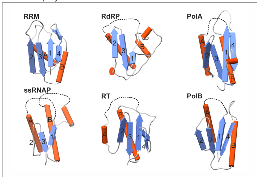
Fig. 1. The core catalytic domains of DNA and RNA polymerases. a Double-psi beta-barrel (DPBB) polymerases. RNAP, multisubunit DNA-dependent RNA polymerase from Thermus thermophilus (PDB ID: 1iw7); eRdRP, eukaryotic RNA-dependent RNA polymerase from Neurospora crassa (PDB ID: 2j7n); PolD, DP2 subunit of family D DNA polymerase from Pyrococcus abyssi (PDB ID: 5ijl). b RRM-fold polymerases. RRM, RNA-recognition motif-containing RNA-binding domain of human nucleolin TIAR (PDB ID: 2cqi); RdRP, RNA-dependent RNA polymerase of poliovirus type 1 (PDB ID: 1ra7); PolA, family A DNA polymerase from Thermus aquaticus (PDB ID: 1taq); ssRNAP, single-subunit DNA-dependent RNA polymerase of bacteriophage T7 (PDB ID: 1msw); RT, reverse transcriptase of Moloney murine leukemia virus (PDB ID: 1mml); PolB, family B DNA polymerase from Thermococcus gorgonarius (PDB ID: 1tgo). c PolC-like polymerases. Polβ, DNA polymerase β from Rattus norvegicus (PDB ID: 1bpb); PolC, family C DNA polymerase from Thermus aquaticus (PDB ID: 2hpi). In b and c , the major secondary structure elements forming the core palm domain are indicated with numbers (for β-strands) and capital letters (for α-helices). Dashed lines indicate regions where insertions into the core palm domains have occurred; these have been omitted for visualization purposes
