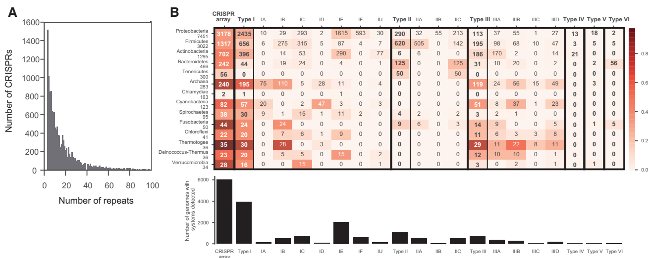
Figure 1. Distribution of CRISPR arrays and clusters of cas genes in the genomes of Prokaryotes. (A) Histogram of the number of repeats in CRISPRs (histogram truncated at 100, because higher values are very rare, maximum is 587). (B) Distribution per clade (on the top panel only clades with >25 genomes are indicated). The cells indicate the number of genomes with systems detected in the clade, and the colour of the cell is proportional to the average frequency per genome (the darker, the more frequent, see scale). The bottom panel shows the total number of genomes with elements detected in the dataset.
