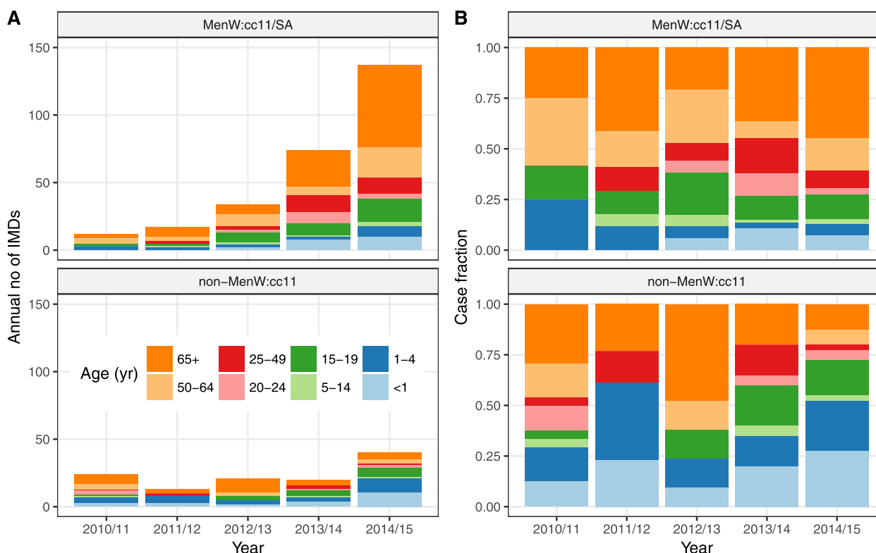
Fig. 1 Incidence of MenW IMDs in England, 2010/2011–2014/2015. Annual number (a) and age distribution (b) of cases caused by MenW:cc11/SA and by other MenW not belonging to cc11 (non-MenW:cc11)
