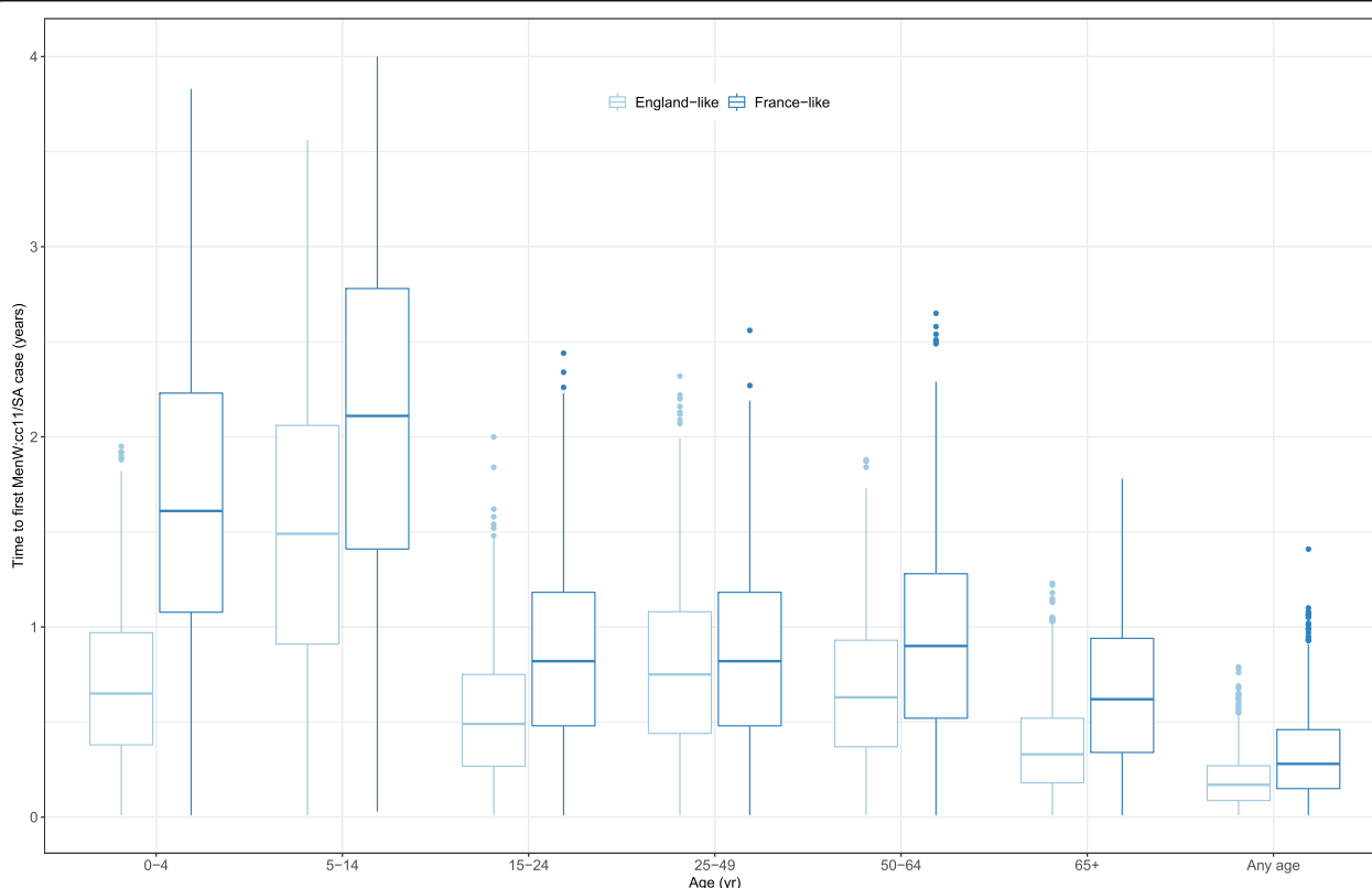
Fig. 5 Predicted duration of silent MenW:cc11/SA carriage transmission. Assuming perfect (i.e., complete and not delayed) reporting, we ran 10^3 model simulations and recorded the time between the start of MenW:cc11/SA carriage transmission and the first report of disease, in a given age group or in any age group. In all simulations, the MenW:cc11/SA parameters used were those estimated in England (Table 2), while the non-MenW:cc11 parameters were fixed to the values calibrated in England (England-like scenarios) or in France (France-like scenarios)
