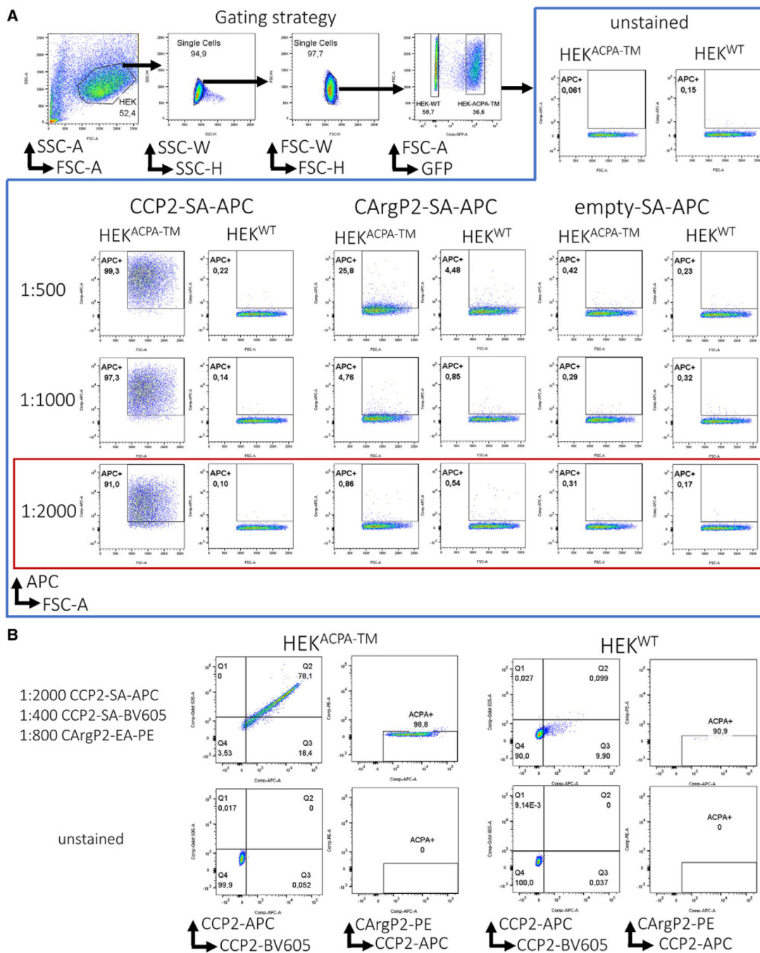
Figure 146. Determining optimal concentrations of multimerized antigen-tetramers for staining. (A) titration of CCP2-SA-APC, CArgP2-SA-APC, and of “empty” streptavidin APC tetramers on ACPA-expressing HEK 293T (HEK-ACPA TM ) and wild-type HEK 293T (HEK WT ) cells. Gates are based on unstained controls. The red square marks the optimal concentration of CCP2-SA-APC. (B) Staining of HEK-ACPA TM and HEK WT cells with combinatorial CCP2 and CArgP2 tetramers.
