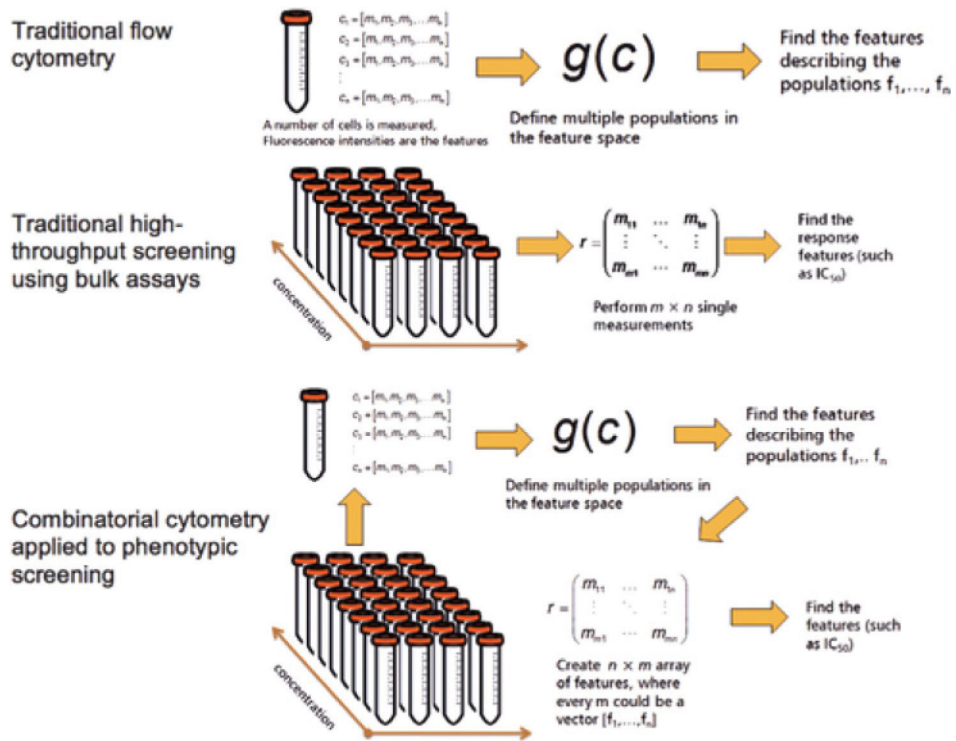
Figure 227. Combinatorial cytometry integrates the ideas of screening biological responses. Biological responses can be screened across multiple conditions (e.g., concentration, medium type, stress, temperature, time, etc.) with FCM. The technique is enabled by fast autosamplers, and informatics pathways aware of the multifactorial nature of the collected data.
