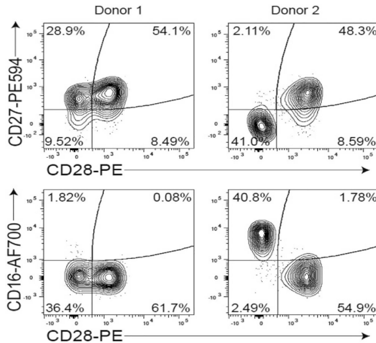
Figure 130. Functional sub-populations of human V\delta 2^+/V\gamma 9^+ T cells. After using the gating strategy to define human \gamma\delta T cells described in Fig. 129, human V\delta 2^+/V\gamma 9^+ T cells can be further split into effector subsets based on CD27, CD28, and CD16 expression. These populations are highly variable between individuals and it is unclear how these populations are derived.
