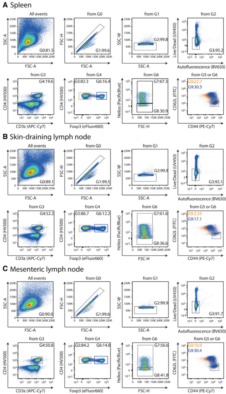
Figure 97. Phenotyping of Treg cells from murine spleen and lymph nodes. (A) Gating strategy to identify Treg cells in the spleen. From all events, lymphocytes can be distinguished by their FSC/SSC properties (gate G0). Based on G0, doublets are excluded twice (gates G1 and G2) followed by exclusion of dead or autofluorescent cells (gate G3). From G3, CD4 + CD3e + T cells (gate G4) are gated, from which Foxp3 + Treg cells (gate G6) and Foxp3 - Tcon cells (gate G5) can be further identified. From G6, Helios + tTreg (gate G7) and Helios - pTreg cells (gate G8) are gated. Finally, a staining for CD62L and CD44 on Treg cells (gate G6,
