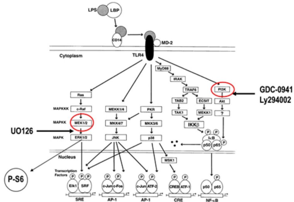
Figure 55. “Canonical” pathways for LPS activation of multiple signaling pathways in peripheral blood monocytes via TLR-4 (adapted from Guha and Mackman [524] and reproduced with permission). Inhibition of PI3K (right) by Ly294002 or GDC-0941) or of MEK 1/2 (left) by UO126 is also illustrated here. Also shown, in monocytes, activation of the ribosomal S6 protein is predominantly through activated ERK.
