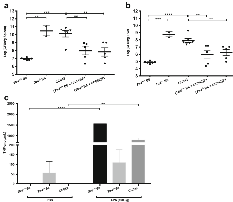
Fig. 6 Tlr4 gene functional study in CC042/GeniUnc. Splenic (a) and liver (b) bacterial loads at day4 p.i. in Tlr4 +/+ B6 ( n = 6), Tlr4 -/- B6 ( n = 2), CC042 ( n = 6), ( Tlr4 +/+ B6 × CC042)F1 ( n = 5) and ( Tlr4 -/- B6 × CC042)F1 ( n = 5) mice infected with 10 3 CFUs of S. Typhimurium (cumulative results from 2 distinct experiments). The TNF-α levels production at 90 min post-mock-PBS injection or 100 μg LPS injection (c) in Tlr4 +/+ B6 ( n = 4 and 4), Tlr4 -/- B6 ( n = 4 and 4) and CC042 ( n = 4 and 5) mice. The values are means and error bars present standard error of mean. Mean bacterial loads (a) and (b) were compared by one-way ANOVA and Tukey HSD test. Mean TNF-α values (c) were compared by two-way ANOVA and Holm-Sidak test. Asterisks indicate respective P-value of P < 0.1 (*), P < 0.01 (**), P < 0.001 (***), P < 0.0001 (****)
