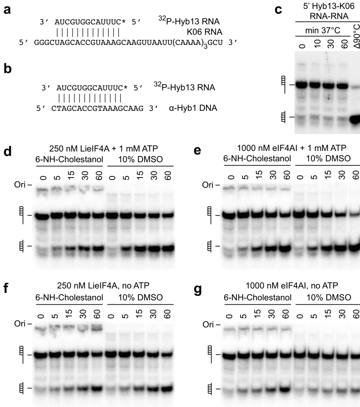
Fig. 2. The helicase activity of LieIF4A. (a) The helicase substrate was made by hybridizing a 13-nucleotide-long RNA (Hyb13) that was labeled on the 5' end with 32 P (*) with a 45-nucleotide-long template RNA (K06) that was not labeled. (b) The Hyb13 released during the helicase reaction was "trapped" by a complementary DNA oligonucleotide (α-Hyb1) that was present at 20-fold excess of Hyb13. (c) The duplex was stable under the reaction conditions in the absence of LieIF4A. However, samples heated to 90 °C formed ≥95% of the Hyb13-α-Hyb1 duplex that migrated faster than the Hyb13-K06 duplex on a 15%, nondenaturing, polyacrylamide gel run at 4 °C. (d) LieIF4A at 250 nM unwinds 50 nM of the duplex in the presence of 1 mM ATP in a time-dependent fashion (shown in minutes). All reactions were done in the presence of 10% DMSO. Ori, indicates the position of the bottom of the wells. In the presence of 100 μM 6-aminocholestanol, a small amount of 32 P-Hyb13, or a complex thereof, migrated as a much higher molecular weight species. (e) An equivalent unwinding
