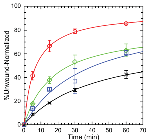
Fig. 4. Normalized mean unwinding activity of LieIF4A and eIF4AI Mus ±10% DMSO. Reactions were done in the presence or absence of 10% DMSO and 1 mM ATP. The mean and standard deviations are shown for three or more independent experiments. Blue □, LieIF4A; red ○, LieIF4A with 10% DMSO; black ×, eIF4AI Mus ; green ◇, eIF4AI Mus with 10% DMSO.
