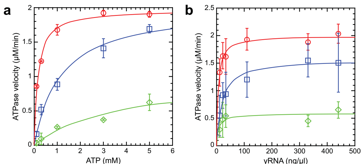
Fig. 1. ATPase reaction velocities of LieIF4A. The means and standard deviations are shown for three or more independent experiments. The values were fit to the nonlinear Michaelis–Menten equation v = V_{\max}[S]/(K_m + [S]) , where [S] is the substrate concentration, K_m is the Michaelis–Menten binding constant and V_{\max} the maximum reaction velocity, using Kaleidagraph software. All the reactions were done in the presence of 10% DMSO and 820 nM LieIF4A. Red o, no added compound; blue □, 100 μM 6-aminocholestanol; green ◇, 300 μM 6-aminocholestanol. (a) The reaction velocities of LieIF4A with 340 ng/μl RNA and different concentrations of ATP, in the presence or absence of 6-aminocholestanol, are as indicated. (b) The reaction velocities of LieIF4A with 5 mM ATP at different concentrations of whole yeast RNA in the presence or absence of 6-aminocholestanol.
