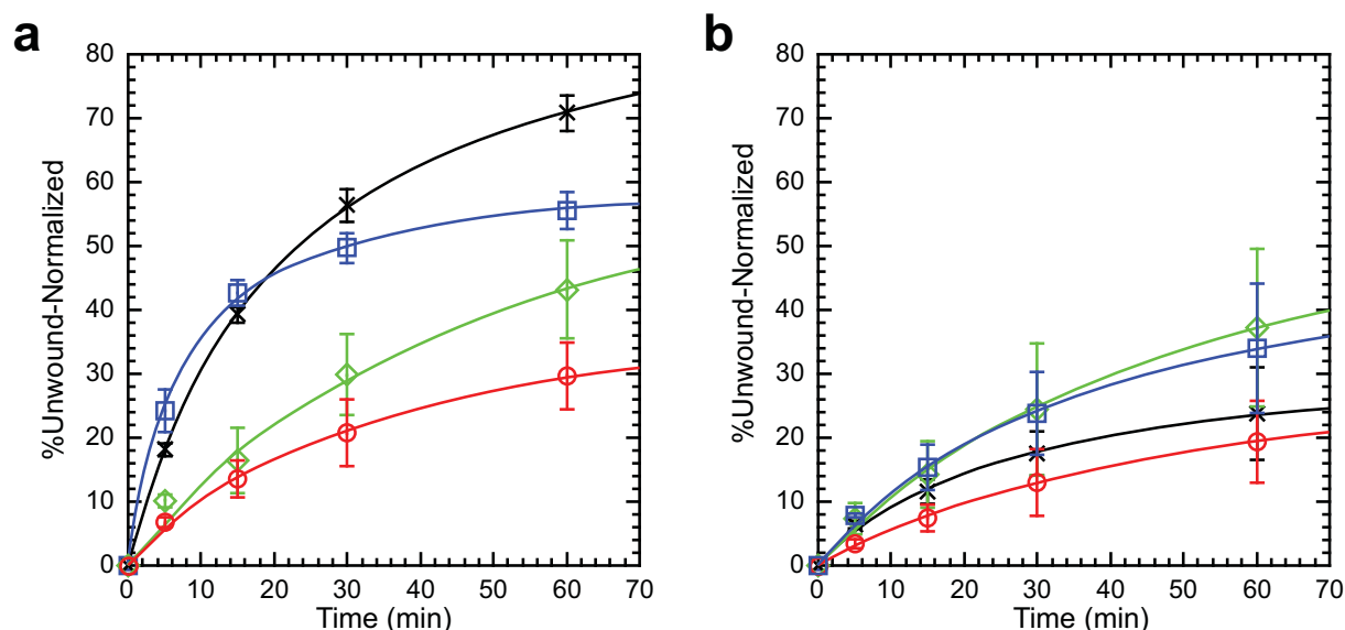
Fig. 3. Normalized mean unwinding activity of LieIF4A and eIF4AI Mus . All reactions were done in the presence of 10% DMSO. The mean and standard deviations are shown for three or more independent experiments. Blue □, LieIF4A; red o, LieIF4A with 100 μM 6-aminocholestanol; black x, eIF4AI Mus ; green ◇, eIF4AI Mus with 100 μM 6-aminocholestanol. (a) The unwinding activities in the presence of 1 mM ATP. (b) The unwinding activities in the absence of ATP.
