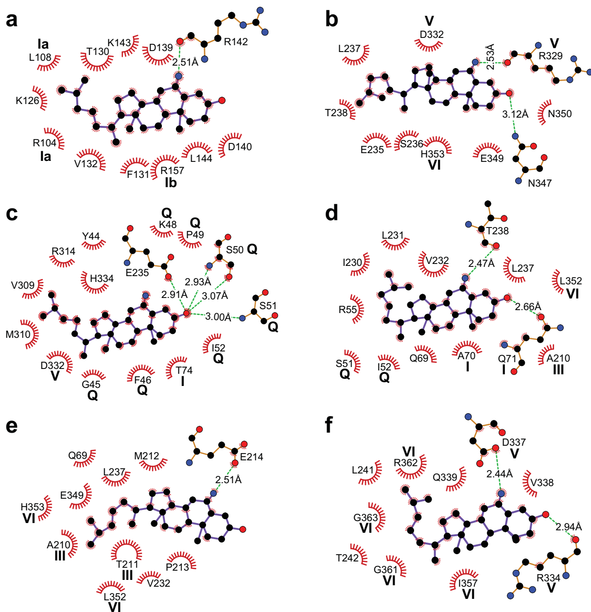
Fig. 5. Interactions of 6- \alpha -aminocholestanol on the identified pockets of LieIF4A and eIF4AI Mus as determined with LigPlot+. Interactions involving residues in conserved motifs are as indicated. The red "brushes" represent van der Waals force interactions and the dotted green lines represent hydrogen bonds. (a) The compound bound in pocket P11 of the open form of LieIF4A. (b) The compound in pocket P19 of the open form of LieIF4A. (c) The compound in pocket P29 of the open form of LieIF4A. (d) The compound bound in pocket P26 of the closed form of LieIF4A. (e) The compound in pocket P39 of the closed form of LieIF4A. (f) The compound in pocket P14 of the open form of eIF4AI Mus .
