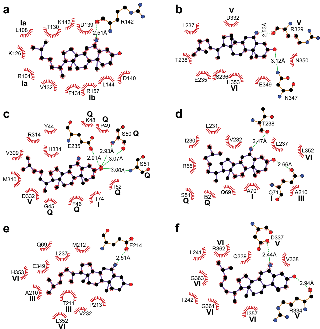
1 2 Fig. 5. Interactions of 6- \alpha -aminocholestanol on the identified pockets of LieIF4A and 3 eIF4A1Mus as determined with LigPlot+. Interactions involving residues in conserved motifs 4 are as indicated. The red "brushes" represent van der Waals force interactions and the dotted 5 green lines represent hydrogen bonds. (a) The compound bound in pocket P11 of the open 6 form of LieIF4A. (b) The compound in pocket P19 of the open form of LieIF4A. (c) The 7 compound in pocket P29 of the open form of LieIF4A. (d) The compound bound in pocket 8 P26 of the closed form of LieIF4A. (e) The compound in pocket P39 of the closed form of 9 LieIF4A. (f) The compound in pocket P14 of the open form of eIF4A1Mus. 10
