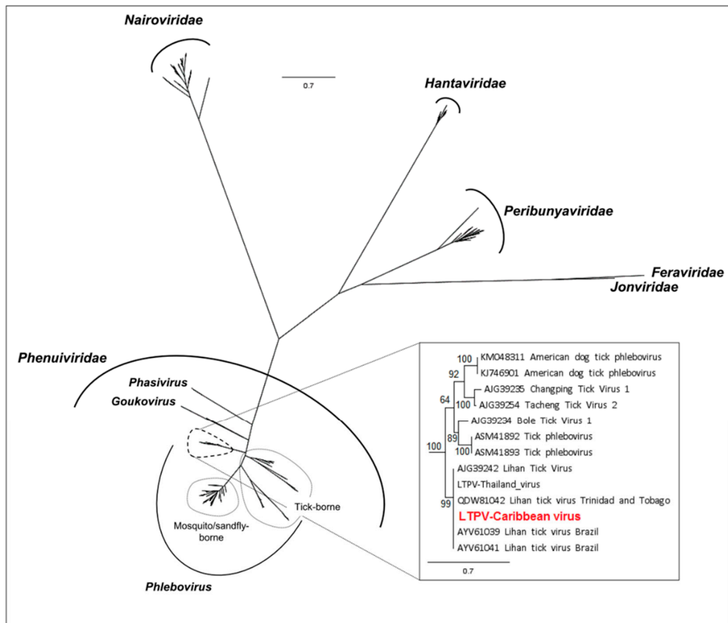
Figure 3. Phylogenetic relationship of Bunyvirales -related viral genomes identified in Caribbean ticks (in red) with other representative viruses ( N = 229 reference sequences). Nodes with bootstrap values greater than 50 are noted. Phylogenetic reconstruction was performed by Maximum Likelihood on the complete RdRP amino-acid gene (model: LG+G+I+F).
