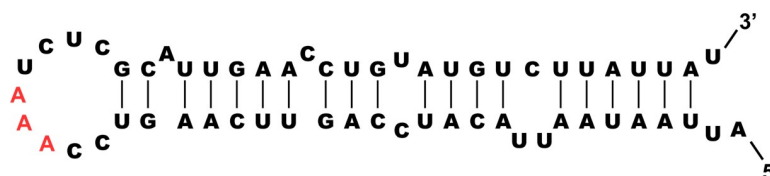
Fig 2. Predicted secondary structure of the cis-acting replicating element of EV-D111. The triplet known to be directly involved in the uridylation of the protein 3B is in red.
