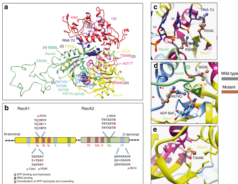
Fig. 2 In silico modeling of DHX37 RecA1 and RecA2 pathogenic variants. (a) Functional domains of a homology model of DHX37 protein with U 7 -RNA (dark blue) and a nonhydrolyzable adenosine triphosphate (ATP) analog (ADP-BeF 3 , spheres). Domains are color-coded and labeled, conserved motifs are specified in circles, and the five disease-associated variants are indicated. The protein has four functional domains: two RecA-like domains, which are the helicase domains (RecA1: ATP-binding DEAH-box helicase, yellow; RecA2: C-terminal helicase, green); helicase associated 2 domain (HA2, red); and oligonucleotide/oligosaccharide-binding domain (OB, pink). (b) Schematic diagram of the RecA-like domains in DEAH-box RNA helicases. Colors represent main helicase functions. Alignment of human (top) and Saccharomyces cerevisiae (bottom) showing the positions of recurrent variants causing 46,XY disorders/differences of sex development (DSD) with the consensus sequence shown in the middle. (c) Zoomed-in view of residue 308 and 334 with single-stranded RNA. (d) Residues 626 and 674 are shown to interact with the ATP analog. (e) Residue 304 is highlighted to be buried with a pocket within the RecA1 domain. Dashed lines within figure parts are shown for selected noncovalent polar interactions.
