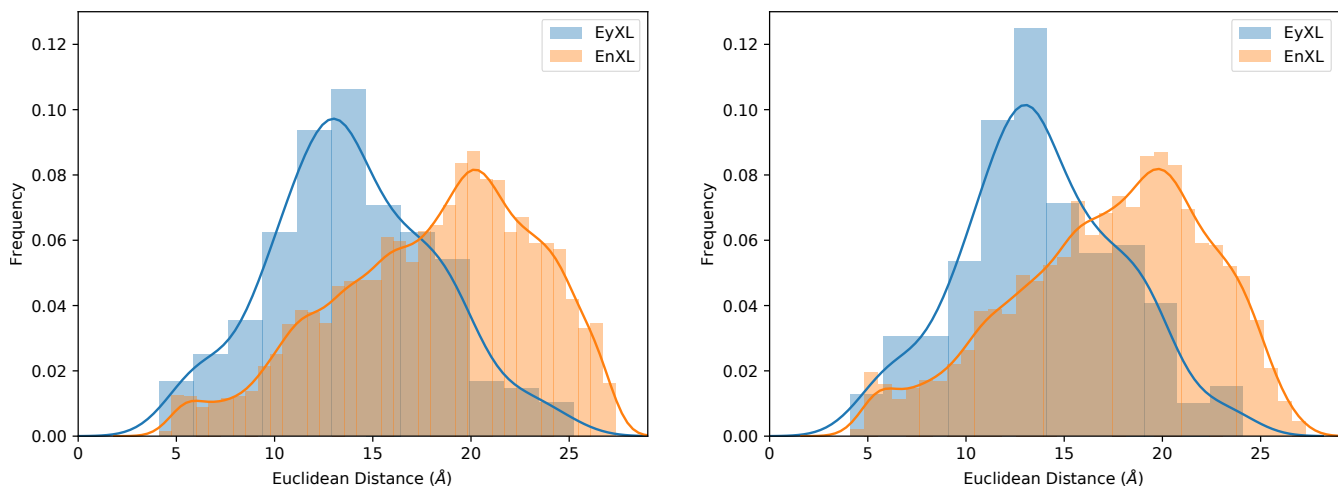
Figure 3. Euclidean distance distributions
