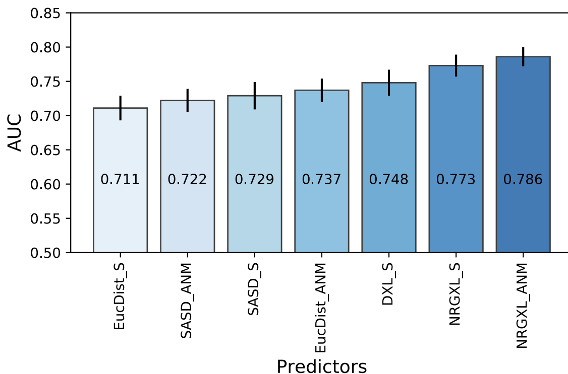
Figure 5. AUC from different statistics and different models
