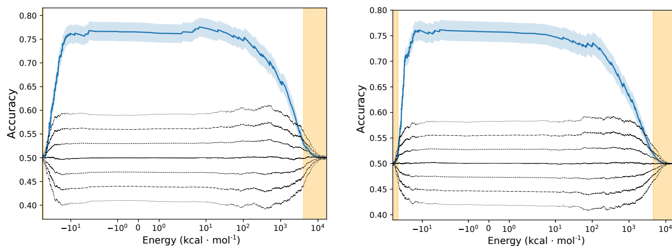
Figure 6. Mean accuracy for different energy thresholds of both the static and the flexible model on a training subset.
