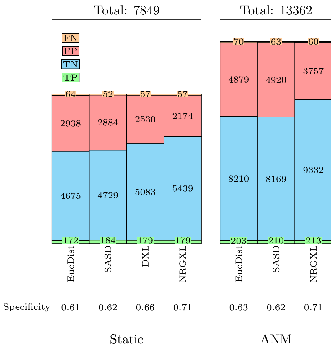
Figure 7. Plain outcomes for Binary Classification studies.
