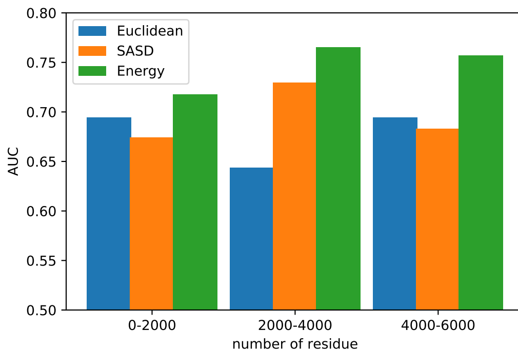
Figure S1. Effect of the protein size on different classifier performance. Related to Figure 5
