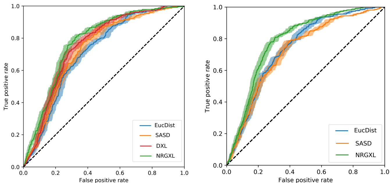
Figure 4. ROC plots for different statistics
