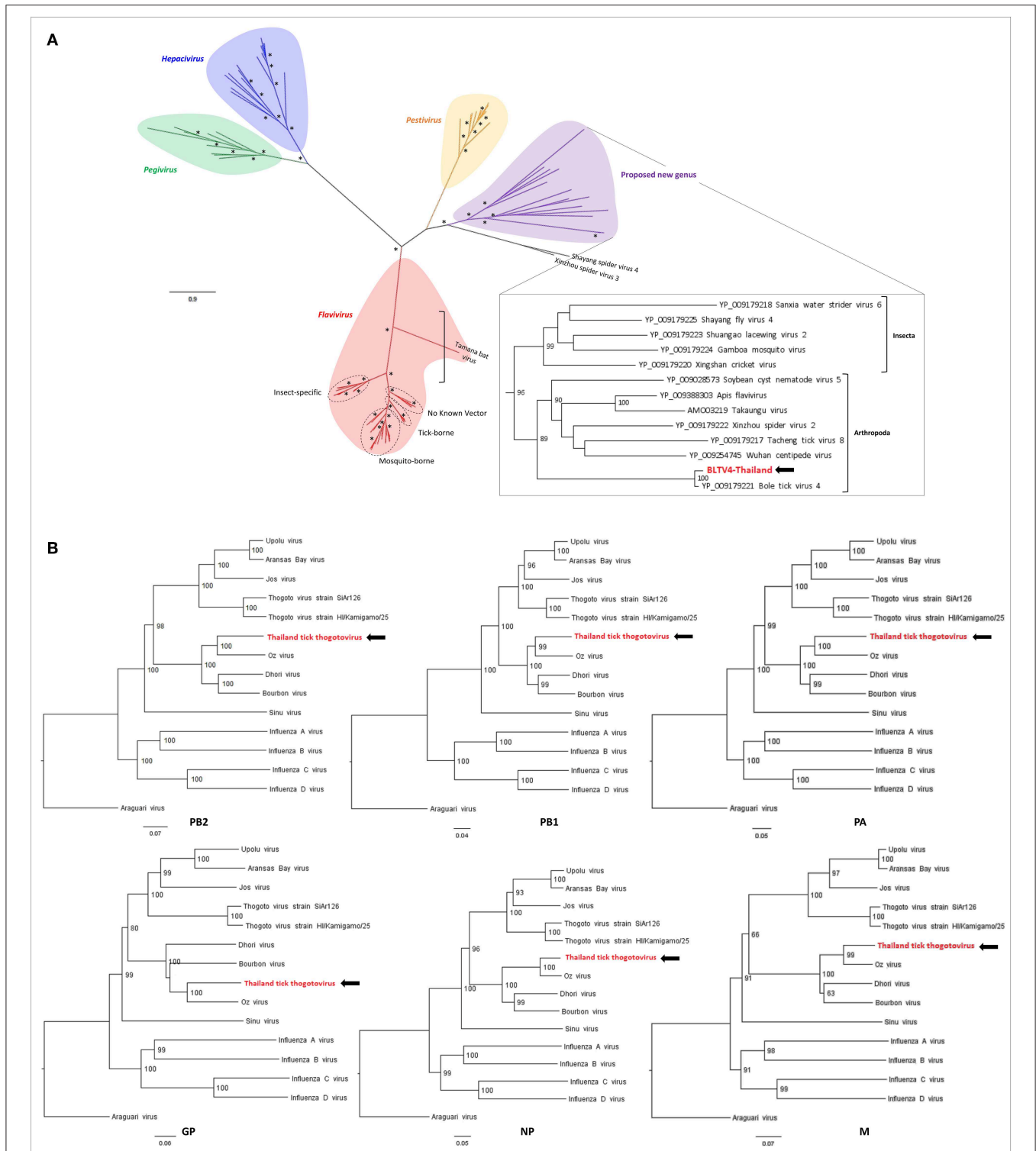
FIGURE 4 | Phylogenetic relationship of viral genomes identified in Thai ticks with other representative viruses. (A) Maximum likelihood (ML) tree of the complete RNA-dependent RNA polymerase (RdRP) amino-acid sequence of representative Flaviviridae viruses (model: LG + G + I + F). Nodes with bootstrap values >50 are noted with an asterisk. (B) Neighbor joining (NJ) trees of the complete PB2–PB1–PA–GP–NP–M amino-acid sequences of representative Orthomyxoviridae viruses (model: p -distance).
