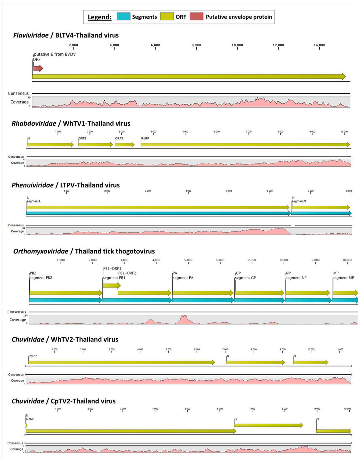
FIGURE 1 | Schematic organization of the six viral genomes identified in Thai ticks. The open reading frames (ORFs) are indicated with yellow arrows, and genome coverage is indicated in pink. Segmented viruses were presented as concatenated sequences for better clarity (blue arrows represent the different segments). The putative envelope glycoprotein (GP) of Thailand tick flavivirus is highlighted by a red arrow in the polyprotein ORF.
