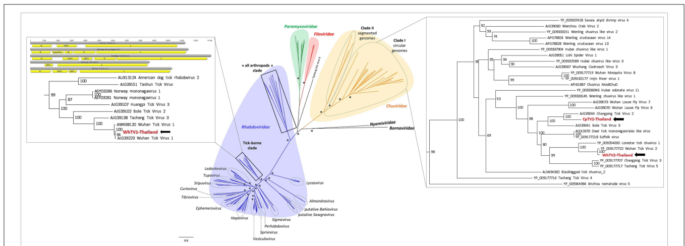
FIGURE 2 | Phylogenetic relationship of Mononegavirales - and Jingchuvirales -related viral genomes identified in Thai ticks with other representative viruses. Nodes with bootstrap values >50 are noted with an asterisk. Phylogenetic reconstruction was performed by maximum likelihood on the complete RNA-dependent RNA polymerase (RdRP) amino-acid gene (model: LG + G + I + F).
