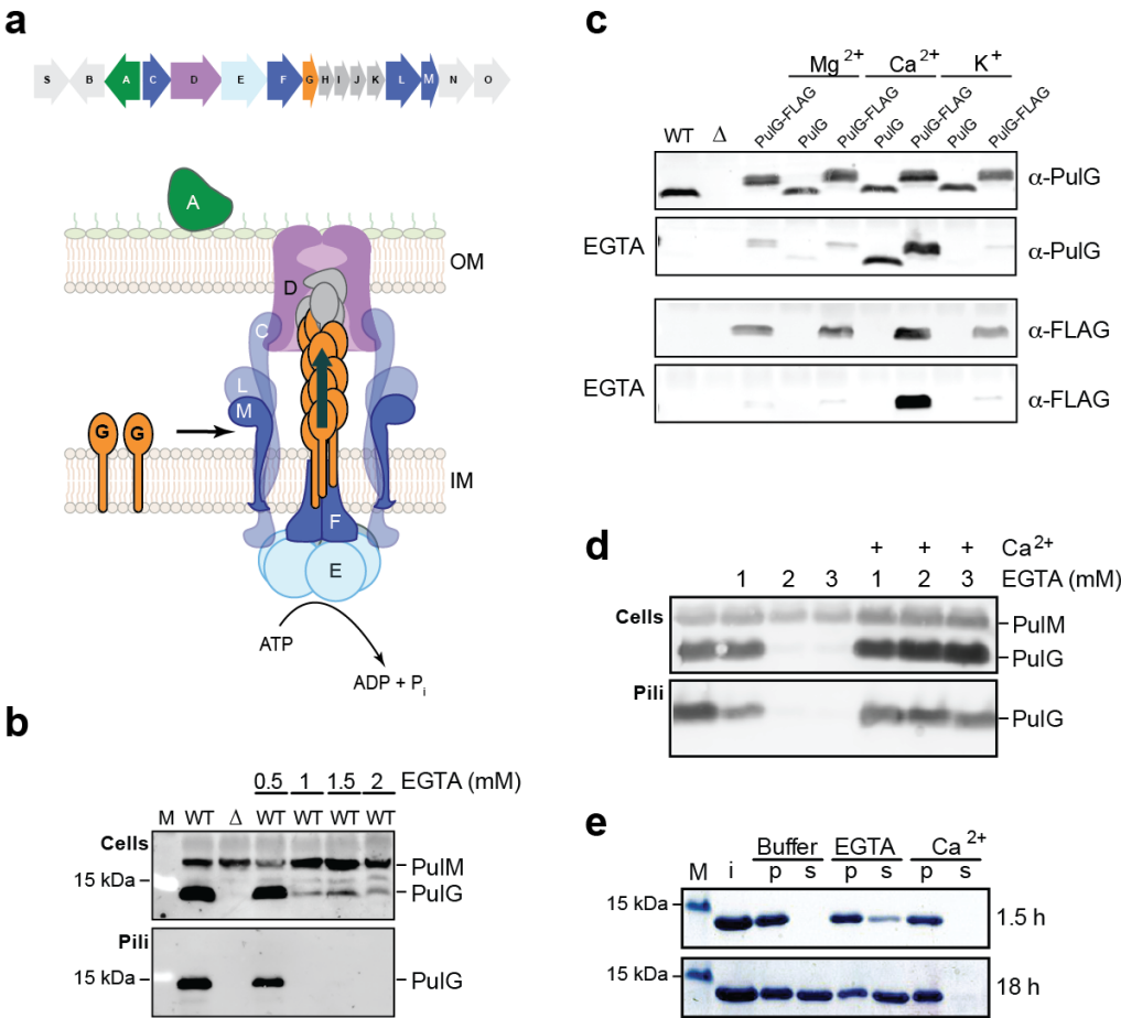
Figure 1. Calcium is required for PulG stability, pseudopilus assembly and stability. a , Top: cartoon of the gene organization in the pul cluster. Bottom: a schematic view of the assembled T2SS nanomachine, with individual components labelled with the corresponding single-letter and colour code. b , c , d , PAP7460 harbouring pCHAP8185 and pSU19 (WT), pCHAP8184 and pSU19 ( \Delta pulG ; \Delta ), pCHAP8184 and pCHAP8658 (PulG), or pCHAP8184 and pCHAP5247 (PulG-FLAG) were grown under pilus-inducing conditions in media supplemented with EGTA and/or cations as indicated. Where appropriate, molecular weight markers (M) are indicated on the left in kDa. b , Effect of EGTA on T2SS function was monitored by probing cell extract and sheared pilus fractions with anti-PulG and anti-PulM antibodies. c , Effect of different cations on total PulG levels was monitored in bacterial cells using PulG ( \alpha -PulG) and FLAG ( \alpha -FLAG) antibodies in absence (top panels) or presence of EGTA (bottom panels). d , Ability of Ca 2+ to restore PulG levels and pseudopilus formation in WT was assessed using anti-PulG and anti-PulM antibodies. e , Pseudopili present on the surface of PAP7460 cells harbouring pCHAP8184 and pCHAP8658 were mechanically sheared and isolated by ultracentrifugation (i). After purification, pseudopili were incubated in buffer alone or buffer supplemented with EGTA or Ca 2+ for the indicated time and intact pseudopili (p) were separated from the supernatant containing broken or degraded pseudopili (s) by ultracentrifugation. All experiments were repeated three times with reproducible results.
