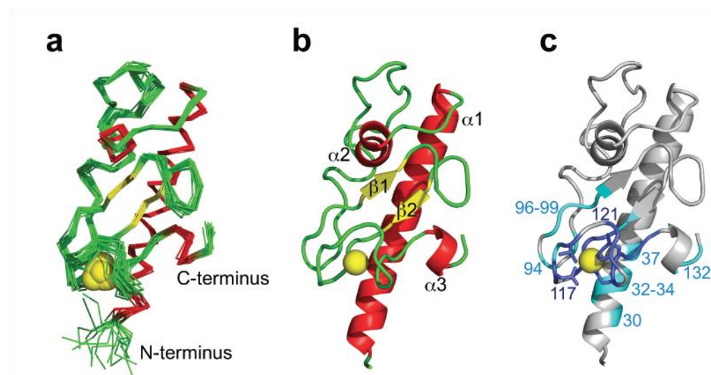
Figure 3. NMR structure of PulGp in the calcium bound state. a , Superposition of the 15 best-calculated structures. b , Ribbon representation of the lowest-energy PulGp conformer. Secondary structure elements are coloured in red (helices) and yellow ( \beta -strands) and calcium atoms are represented as yellow spheres. c , Residues that exhibit significant CSP values (above the dashed line threshold in Fig. 2b) are coloured in dark blue (CSP>0.2 ppm) and light blue (CSP>0.04 ppm) in PulGp structure. For clarity, not all significantly affected residues are labelled. Side chains of some of the calcium-coordinating residues are shown as sticks.
