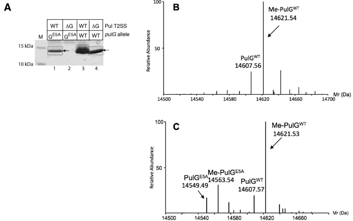
Figure 1. PulG E5A is N-methylated and co-assembled into pili with PulG WT . A. SDS-PAGE and Coomassie Blue stained sheared fractions from equivalent amounts of bacteria of strain PAP7460 carrying two compatible plasmids (Table 1), as indicated: lane 1, pCHAP8185 (encoding the complete Pul T2SS) and pCHAP7790 (encoding PulG E5A ); lane 2, pCHAP8184 (encoding Pul T2SS lacking PulG) and pCHAP7790; lane 3, pCHAP8185 and pCHAP1205 (encoding PulG WT ); and lane 4, pCHAP8184 and pCHAP1205. Only the relevant portions of the gel are shown, with the molecular mass markers indicated on the left. The squares and arrowheads indicate samples that were further analysed by mass spectrometry. B. Deconvoluted high-resolution mass spectrum (in Mr) obtained for the sample in lane 4 (PAP7460 carrying pulG WT allele) indicating the presence of a minor peak at 14607.56 Da corresponding to PulG WT and a major peak at 14621.54 Da corresponding to methylated PulG WT ; C. Deconvoluted high resolution mass spectrum (in Mr) obtained for the sample in lane 1 (PulG WT + PulG E5A ) indicating the presence of supplementary peaks corresponding to PulG E5A (14549.49 Da) and methylated PulG E5A (14563.53 Da).
