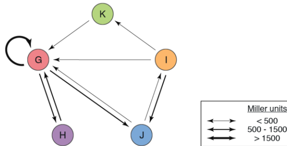
Figure 4. Pseudopilin interaction network determined by the bacterial two-hybrid analysis. A. Beta-galactosidase activities of DHT1 bacteria co-producing indicated T18 and T25 chimera determined as described in Experimental Procedures and expressed in Miller units. NC, activity of bacteria producing T18 and T25 as negative control; PC, activity of positive control strain producing T18-Zip and T25-Zip chimera. Each bar represents mean beta-galactosidase activity value from at least 3 independent colonies obtained by co-transformation of pKT25 and pUT18c derivatives encoding pseudopilin chimera (T25 or T18 fused to the N-terminus of mature pseudopilins) indicated by the colour code in the inset: PulG, red; PulH, purple; PulI, orange; PulJ, blue; and PulK, green. The colours of the bars correspond to the T25-fused proteins. The red horizontal line indicates the background mean beta-galactosidase activity measured in the negative control. Error bars indicate standard deviation. Statistical significance relative to the negative controls is indicated above graphs as follows: **** = p < 0.001 ; *** = P < 0.01 ; * = P < 0.1 ; ns= non-significant. The inset above the main graph shows the part of the same graph with the scale of beta-galactosidase activities expanded in the low range (from 0 to 500 Miller units). B. The results are summarised schematically in a pentagram depicting pseudopilin arrangement in a putative right-handed helical complex. Arrows are oriented from T18- to T25- chimera and their line thickness indicates the strengths of significant interactions, in the range of beta-galactosidase activities (in Miller units) defined as shown in the legend: weak (50>mean>500), strong (500>mean>1500) and very strong (mean>1500).
