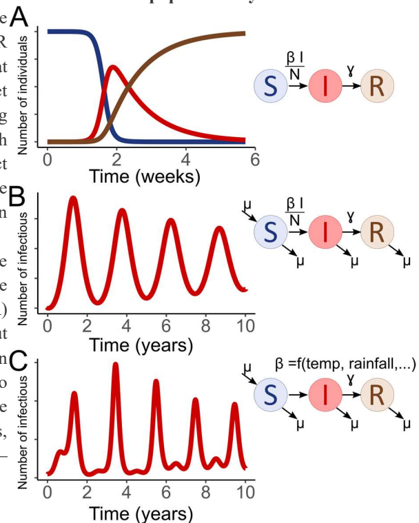
Figure I: Schematics of compartmental models and population dynamics
