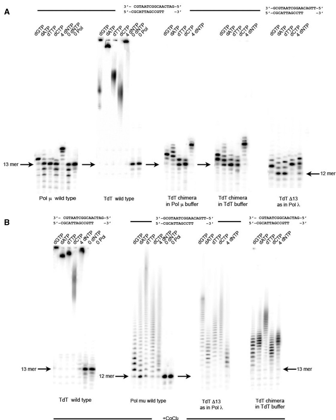
Figure 4. Mimicking pol \mu and pol \lambda with Tdt. (A) The activity without \text{CoCl}_2 but in the presence of 4 mM \text{MgCl}_2 of wild-type Tdt and Tdt Chimera containing the pol \mu Loop1, as well as the \Delta 13 mutant (as in pol \lambda ) is shown for each dNTP and a mixture of all dNTPs. (B) The effect of \text{Co}^{++} addition (1 mM) to the reaction buffer is shown for the same mutants.
