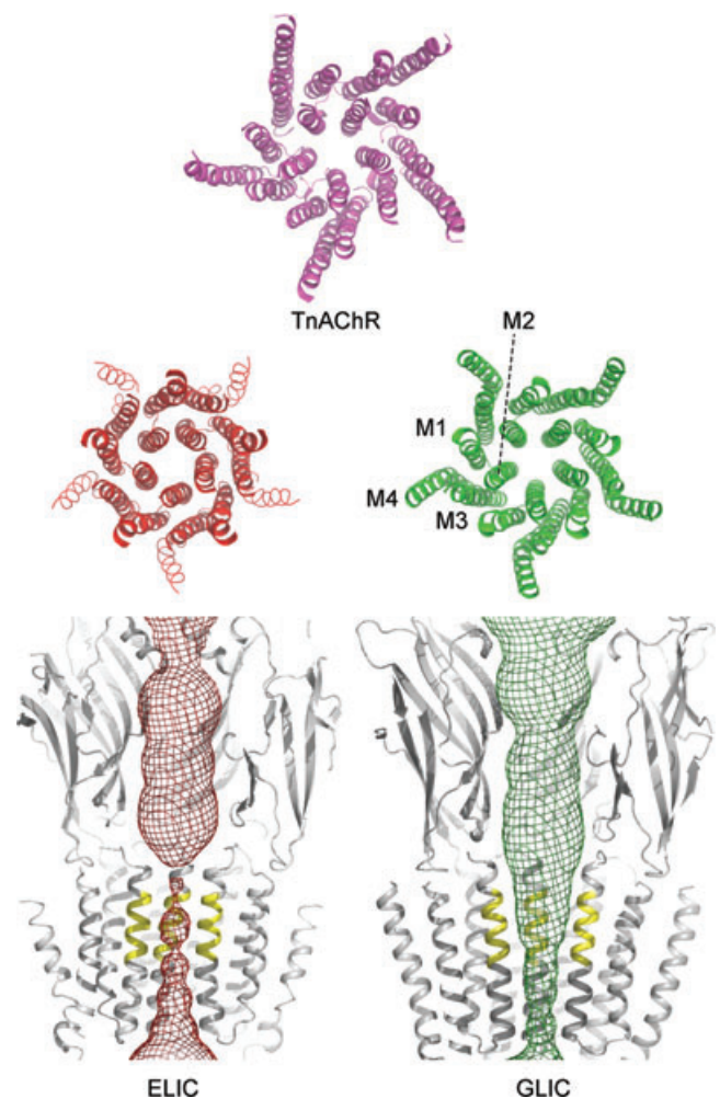
Figure 4. The permeation pathway of GLIC and ELIC Mesh representation of the aqueous pathway in the ELIC and GLIC structures, illustrating that ELIC is in a closed conformation, and GLIC is apparently open. The top view shows the transmembrane helices alone, illustrating that the conformation of the pore and of the M2 helices are similar between GLIC and TnAChR.
