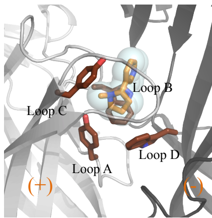
Nicotine-bound Ls-AChBP
