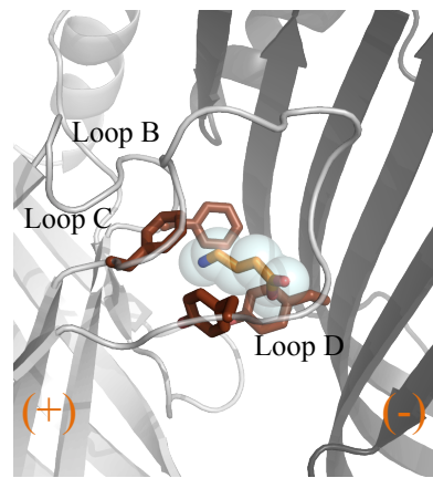
GABA-bound ELIC
