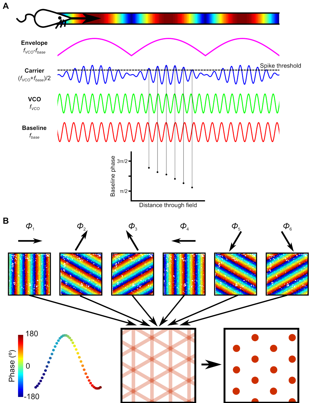
Figure 2: The Oscillatory Interference Model. (A) In 1D, consider a baseline oscillation with frequency f_{base} (red line) and a velocity controlled oscillation (VCO) with a frequency f_{VCO} (green line) that varies linearly with movement speed. Constructive interference between these two oscillations generates a spatially periodic activity pattern with a carrier frequency (blue) equal to their mean frequency (f_{base} + f_{VCO})/2 and an envelope frequency (pink) equal to their difference in frequency (f_{VCO} - f_{base}) . This activity pattern corresponds to spatially periodic, approximately Gaussian firing fields (top) within which spikes are fired at progressively earlier phases of the baseline oscillation (bottom), as observed in grid cells (following Blair et al., 2008). (B) Velocity controlled oscillators (VCOs) with different preferred firing directions \phi_i encode periodic displacement along that direction in their firing phase. Combining input from two or more VCOs with preferred firing directions that differ by multiples of 60^\circ can then account for the periodic firing fields exhibited by grid cells, which fire when their VCO inputs are in phase (adapted from Bush and Burgess, 2014).
