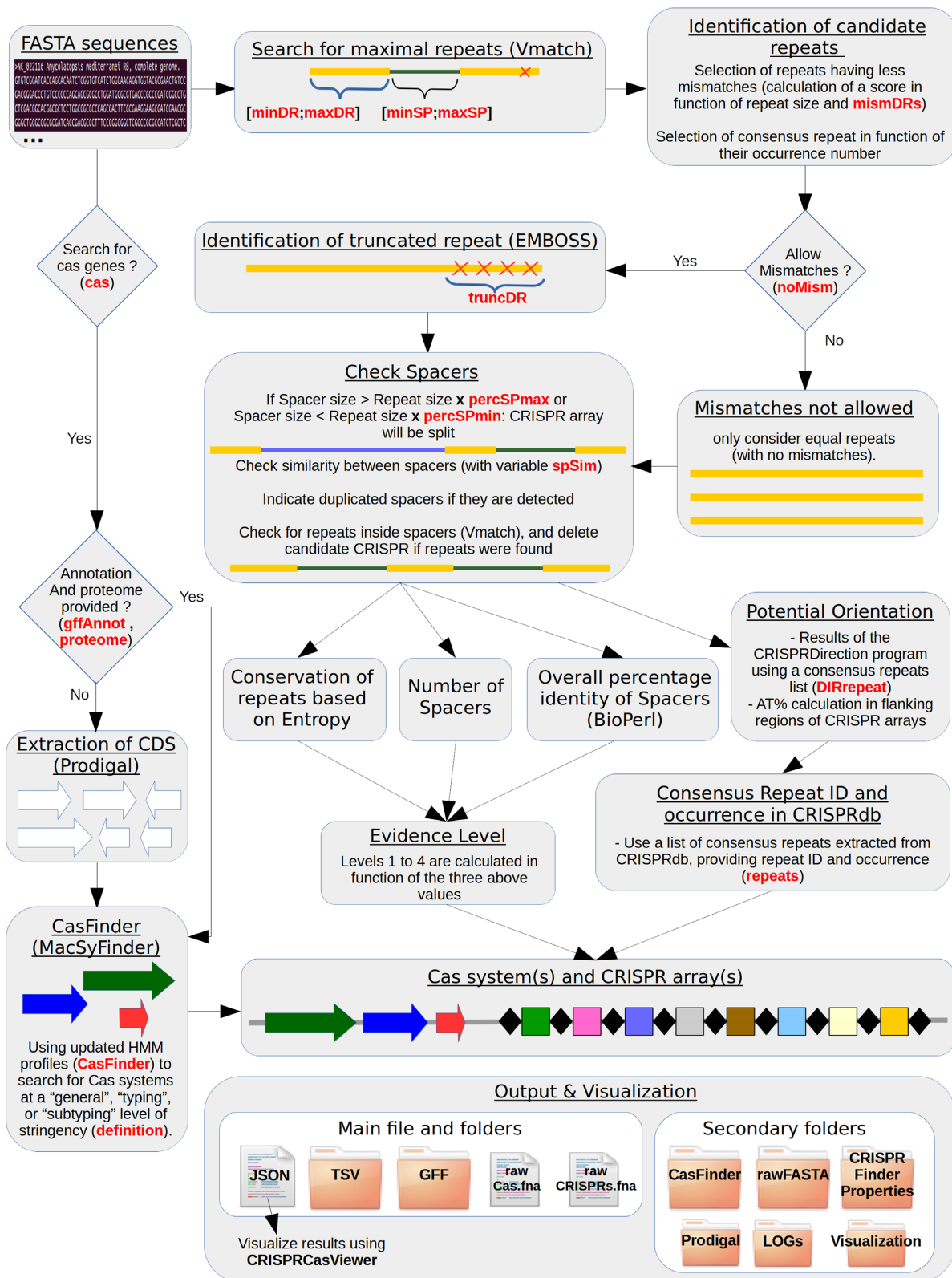
Figure 1. CRISPRCasFinder workflow.
