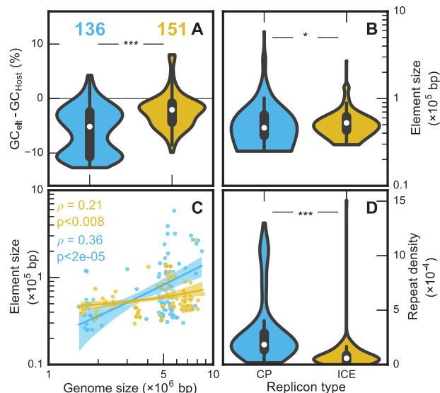
Fig. 1. Comparison between 136 CPs (blue) and 151 ICEs (yellow) in terms of their composition and size. (A) Violin plot showing the distribution of the differences between the elements' GC content and that of their hosts'. CPs are AT richer than ICEs relative to their hosts (Wilcoxon rank sum test, P value < 10^{-3} ). (B) Violin plots showing the distribution of size of ICEs and CPs. ICEs and CPs have different distributions of size (same test, P value < 0.05 ). Median sizes: ICEs (52.5 kb) > CPs (46.1 kb). Averages: ICEs (59 kb) < CPs (74.6 kb) (C) Plot of the size of the element as a function of their hosts' genome size (decreased by the size of the mobile element itself). Shaded regions indicate the 95% confidence interval. (D) Violin plots showing the distribution of the density of repeats in the two types of elements. The density of repeats is higher in CPs than in ICEs (0.30 vs. 0.078 repeats per kb, same test, P value < 10^{-10} ).
