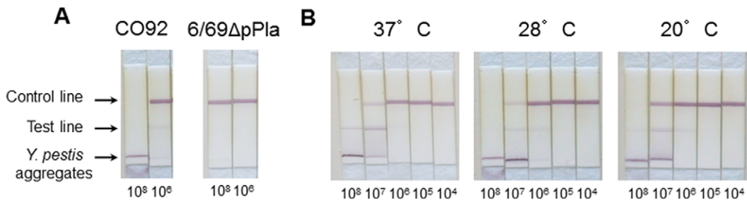
Figure 7. Lateral flow immunoassays. (A) Specificity of the PLA-dipstick for Y. pestis harboring pPla. Both CO92 and 6/69ΔpPla were grown at 28°C and serially diluted. The bacterial suspensions were incubated for 10 min with colloidal gold-labeled Pla35 mAb, and the PLA-dipsticks were then dipped for 30 min into 100 μl of the bacterial suspensions for upward migration of the liquid. Numbers below the dipsticks indicate the number of cfu/well. (B) Influence of the temperature of culture on CO92 detection. Bacteria were grown at 20°C, 28°C or 37°C, and the tests were performed as described in (A). doi:10.1371/journal.pone.0054947.g007
