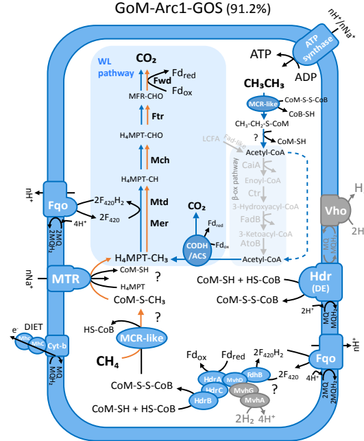
GoM-Arc1-GOS (91.2%)
