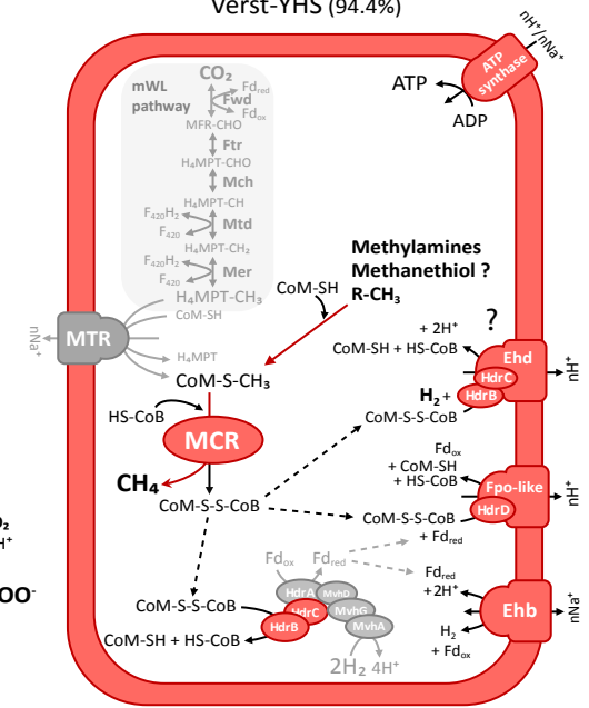
Verst-YHS (94.4%)
